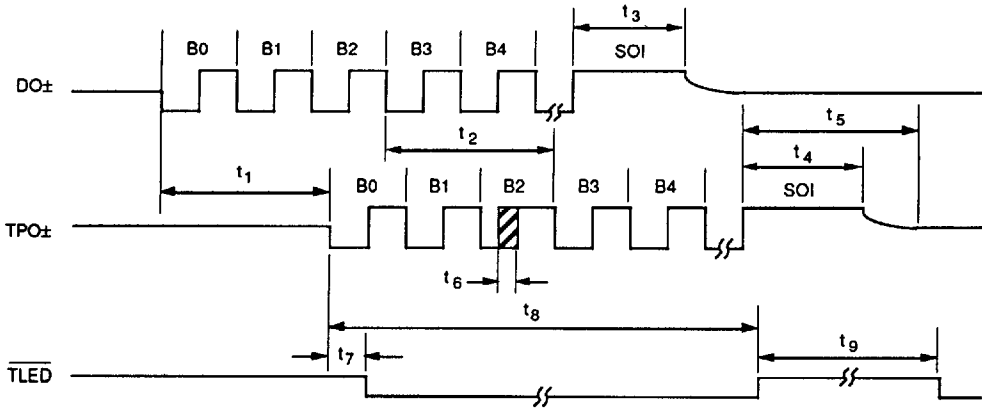
Figure 10. Transmit Section Timing
