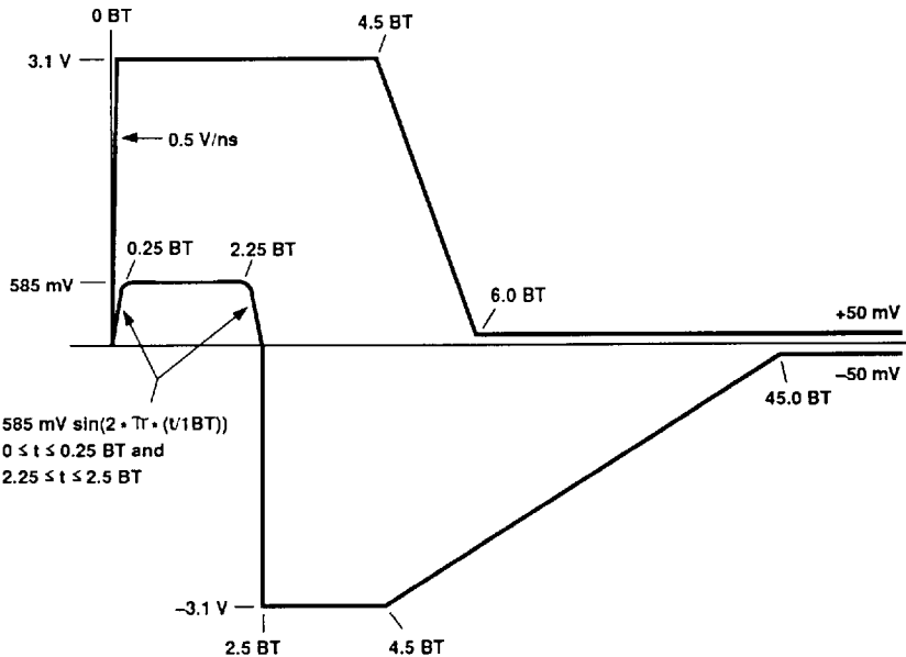
Figure 5. TP Transmit SOI Pulse Voltage Template
