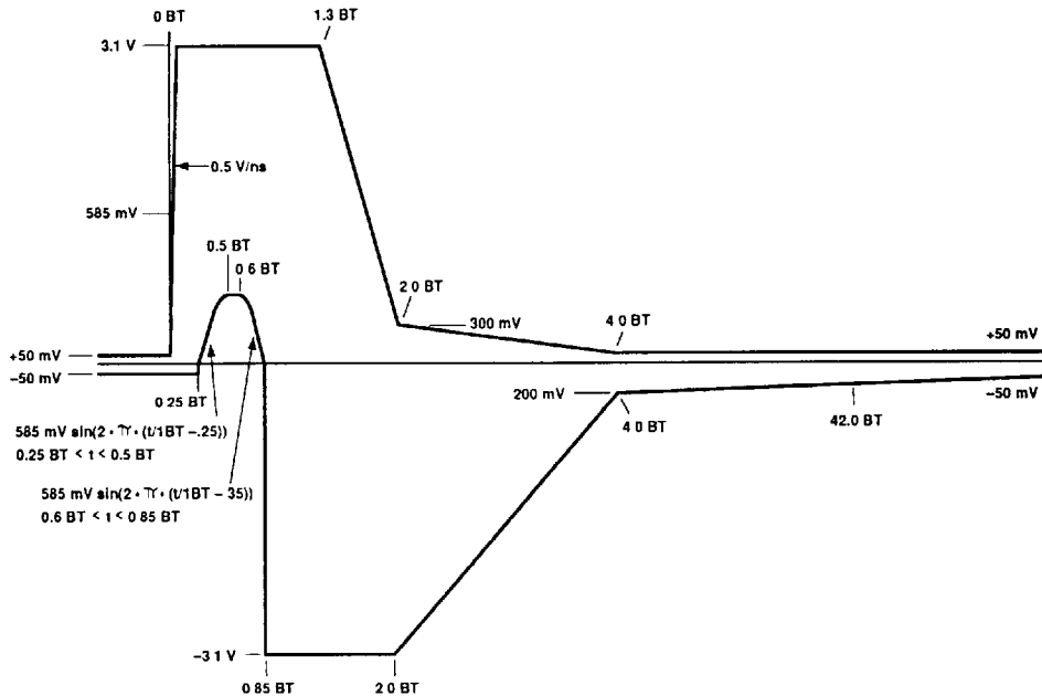
Figure 7. Transmit Link Pulse Voltage Template
