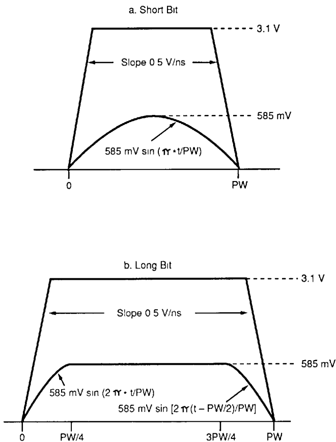
Figure 3. TP Receive Input Differential Voltage Template
