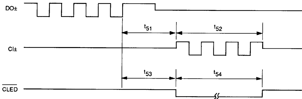
Figure 13. SQE Timing
