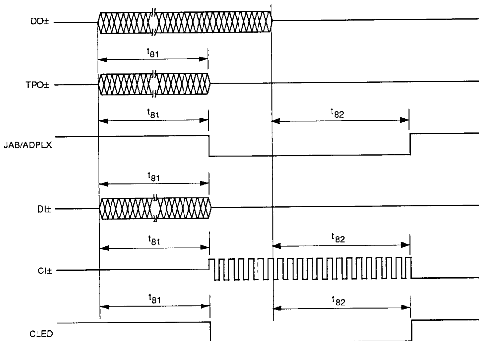
Figure 15. Jabber Timing
