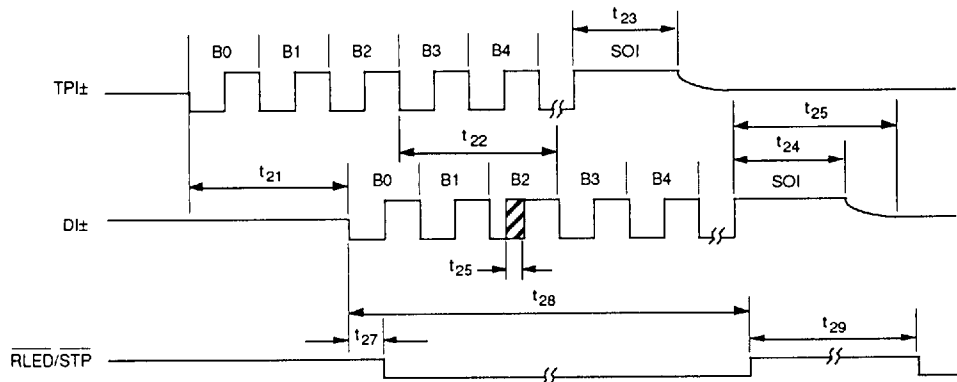
Figure 11. Receive Section Timing
