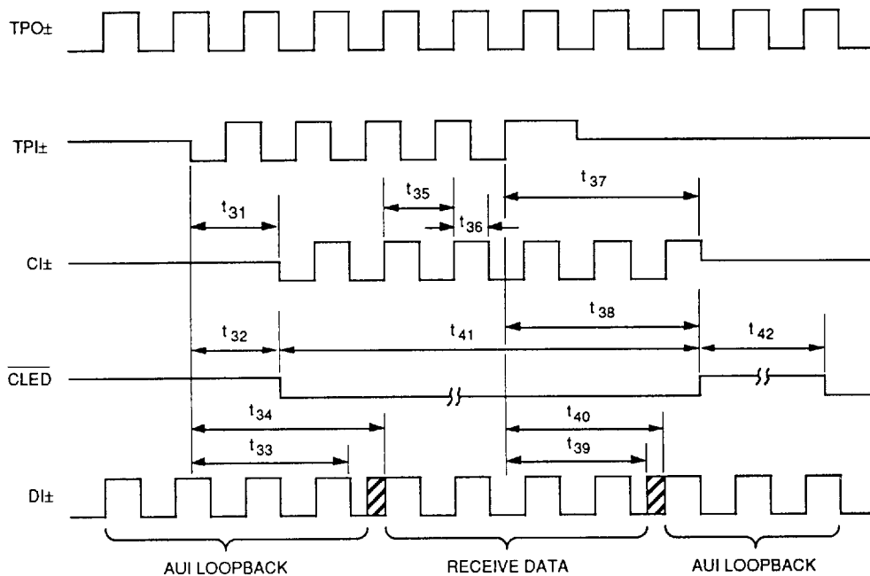
Figure 12. Collision Timing
