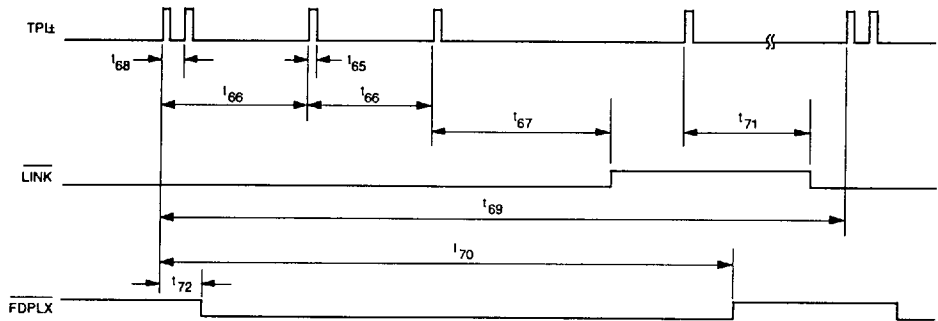
Figure 14. Link Pulse Timing
