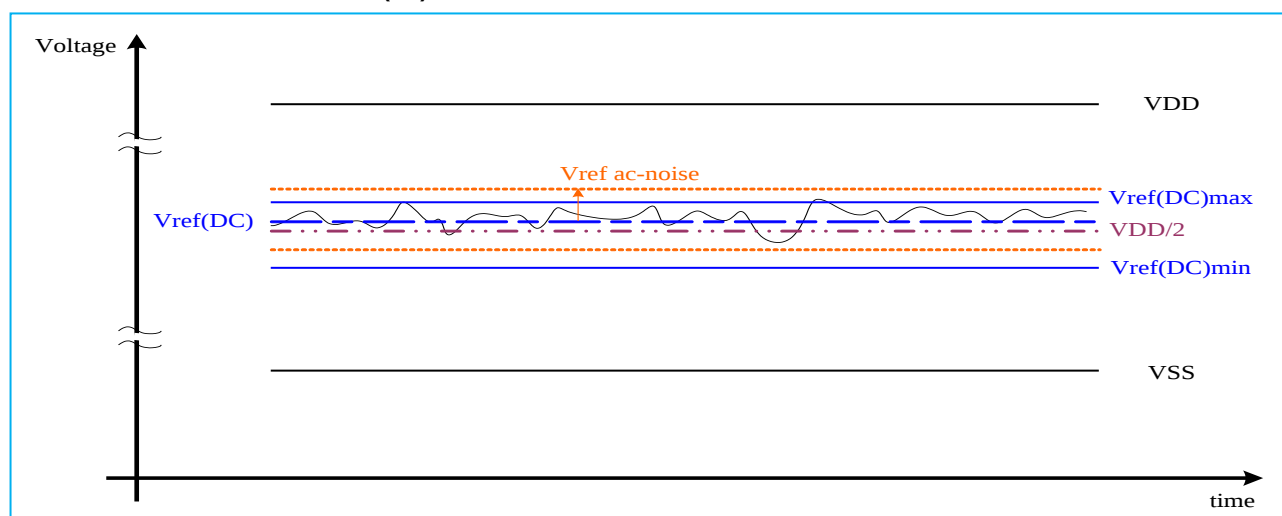
Fig. 60: Illustration of V_{\text{ref}}(\text{DC}) tolerance and V_{\text{ref}} ac-noise limits
