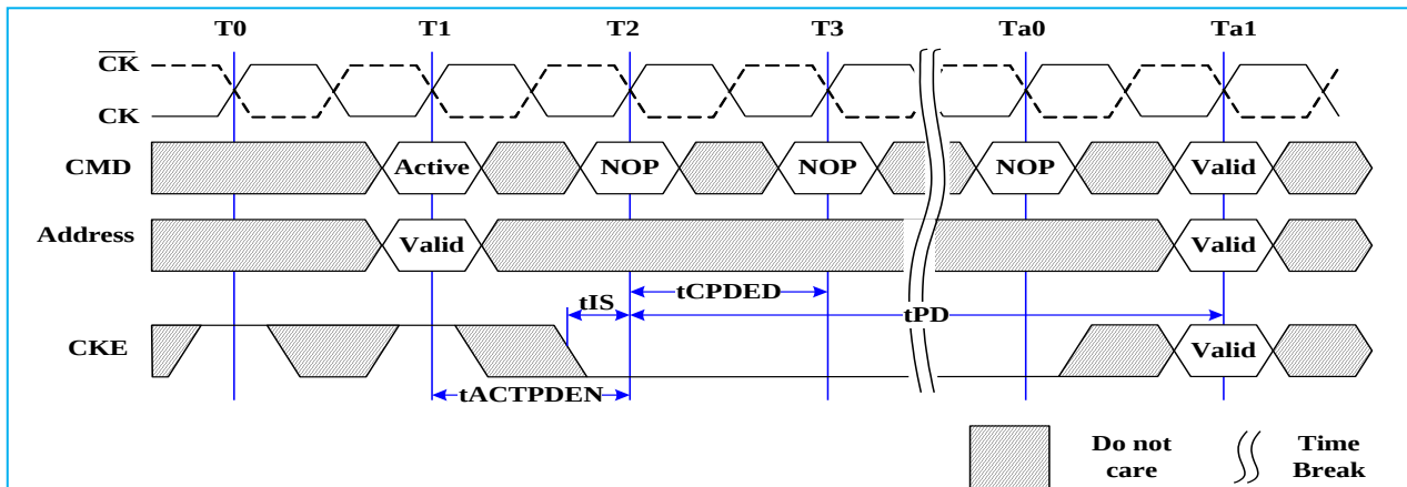
Fig. 43: Active Command to Power-Down Entry
