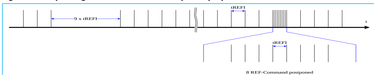
Fig. 33: Postponing Refresh Commands (Example)
