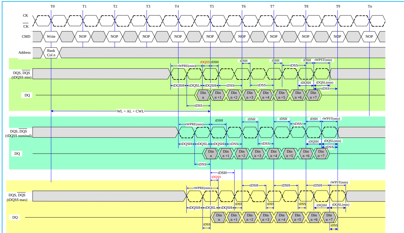
Fig. 28: Write Timing Definition
