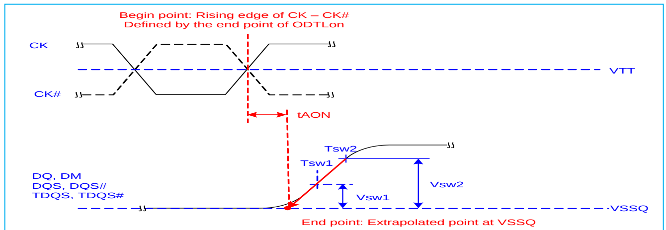
Fig. 69: Definition of t AON
