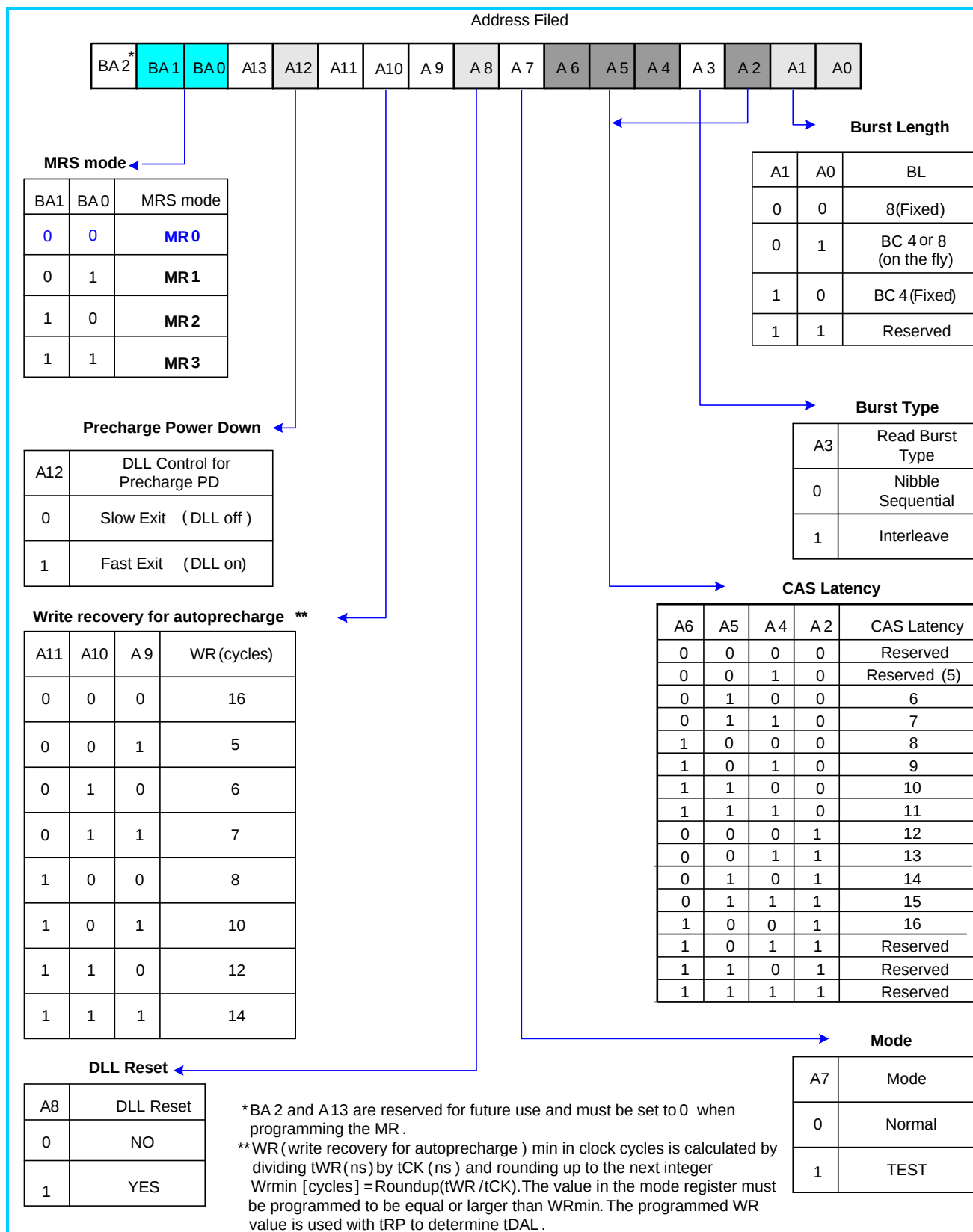
Fig. 8:MR0 Definition
