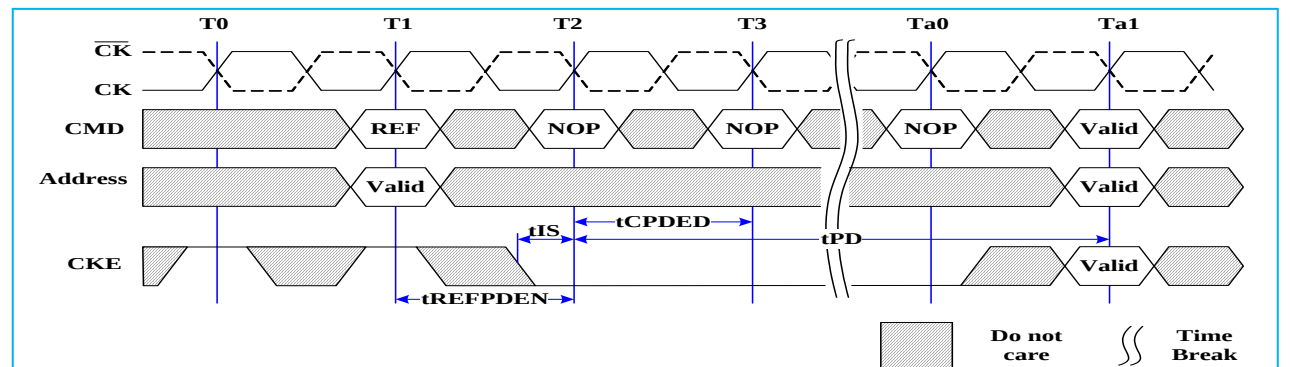
Fig. 42: Refresh Command to Power-Down Entry
