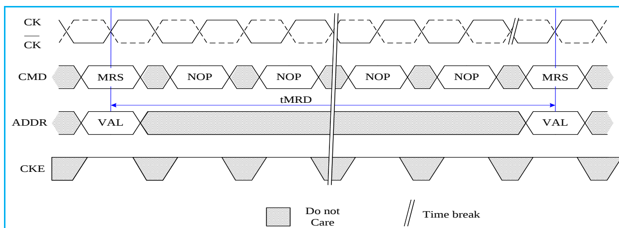
Fig. 6: t_{MRD} Timing
