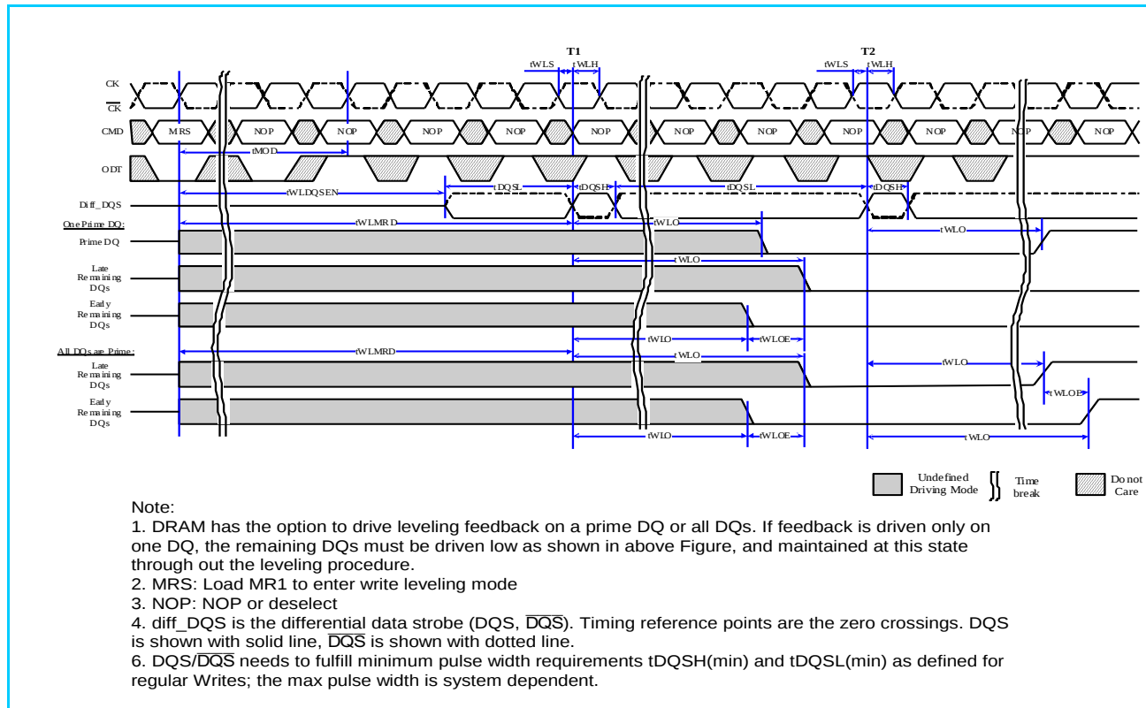
Fig. 18: DQS - \overline{\text{DQS}} is capturing CK - \overline{\text{CK}} low at T1 and CK - \overline{\text{CK}} high at T2
