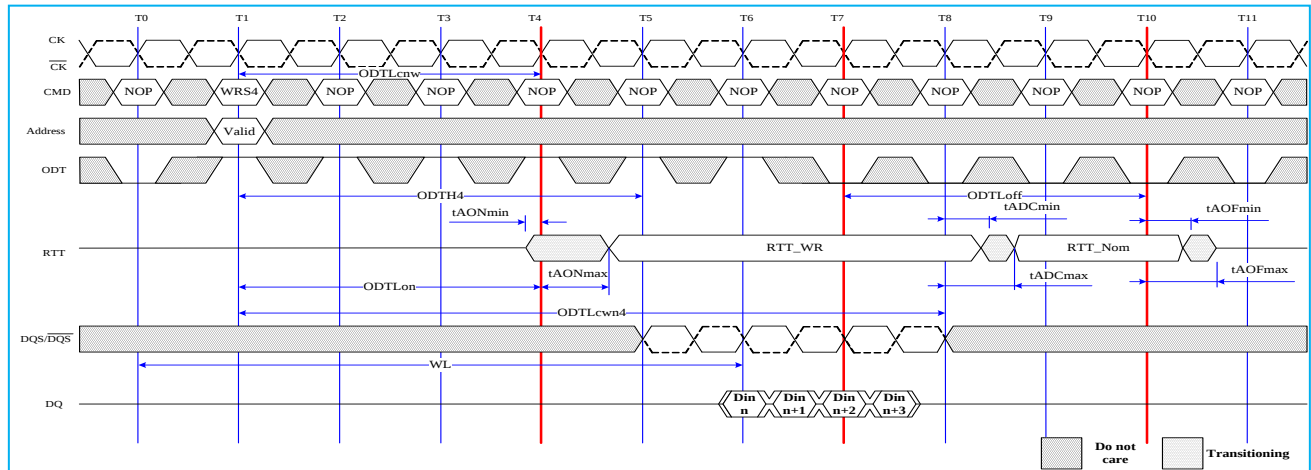
Fig. 53: Dynamic ODT: Behavior with ODT pin being asserted together with write command for a duration of 6 clock cycles, example for BC4 (via MRS or OTF), AL=0, CWL=5.
