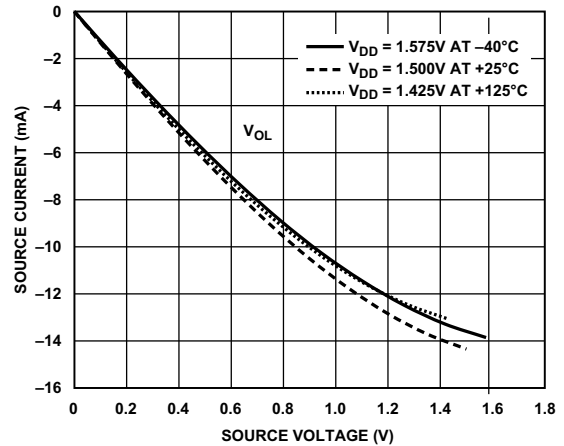
Figure 69. Driver Type B and Driver Type C (DDR3 Drive Strength 100 \Omega )
