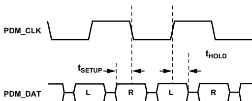
Figure 64. PDM Timing
