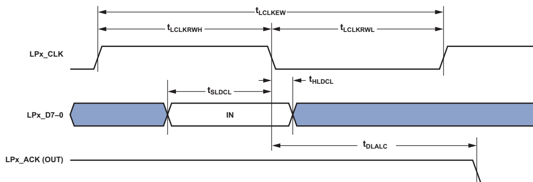
Figure 10. LPs—Receive
