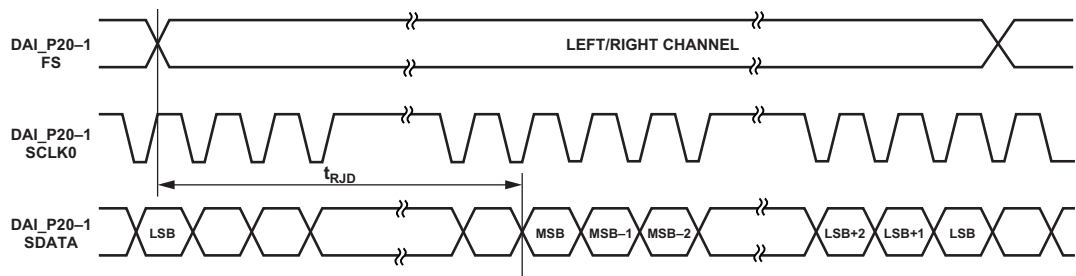
Figure 52. Right Justified Mode
