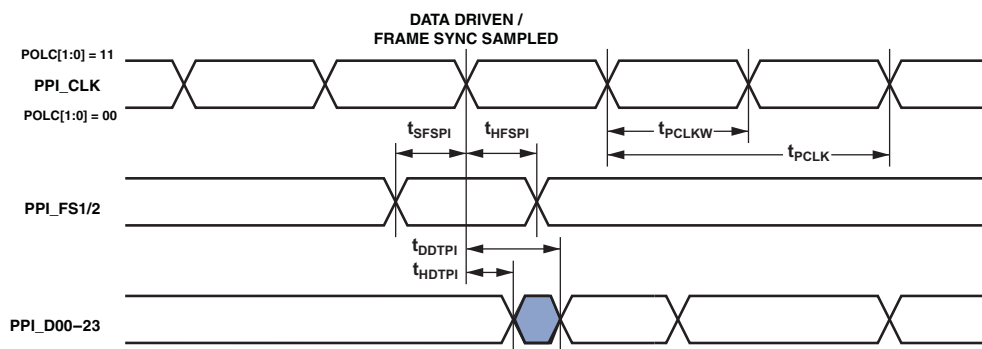
Figure 43. EPPI Internal Clock GP Transmit Mode with External Frame Sync Timing
