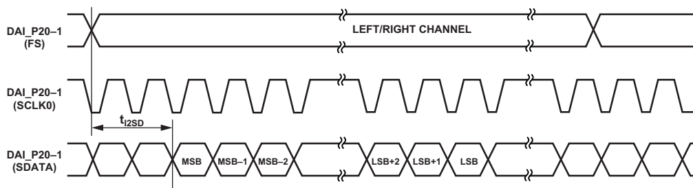
Figure 53. I 2 S Justified Mode
