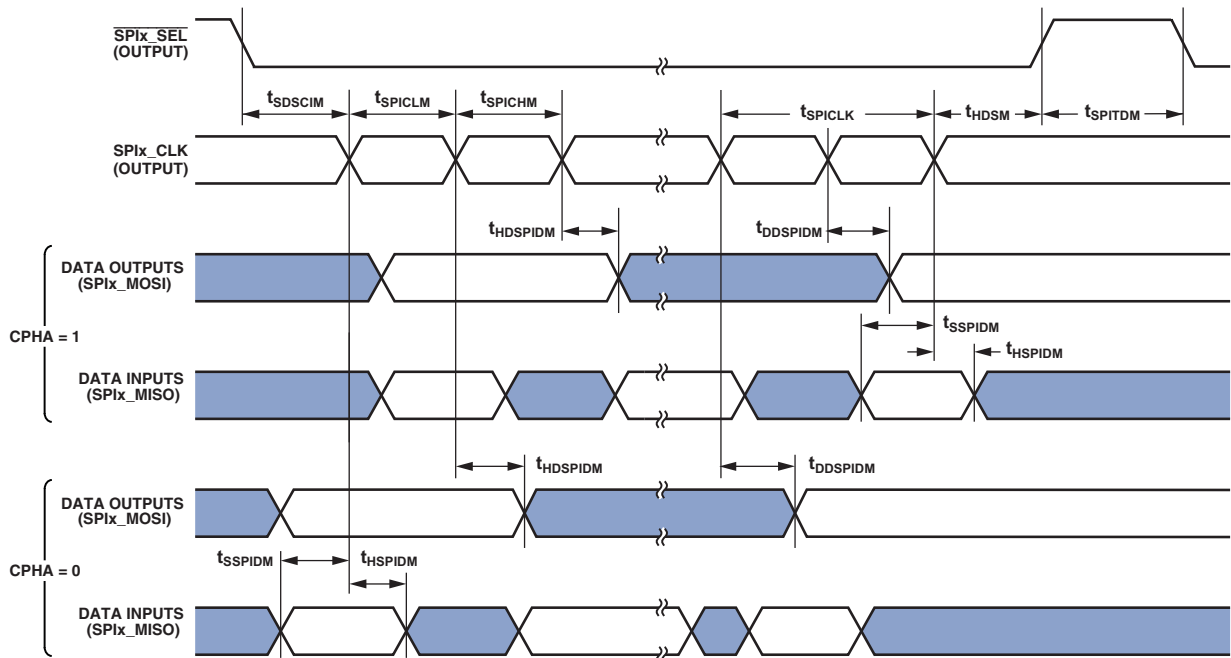
Figure 20. SPI Port—Master Timing
