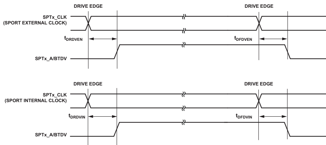
Figure 16. SPORTs—Transmit Data Valid Internal and External Clock
