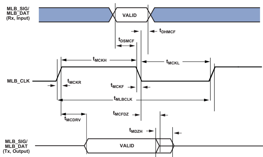
Figure 57. MLB Timing (3-Pin Interface)
