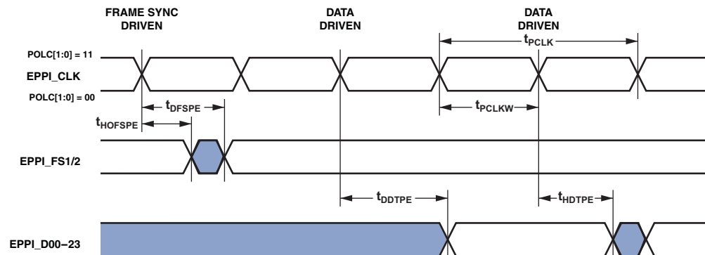
Figure 46. EPPI External Clock GP Transmit Mode with Internal Frame Sync Timing
