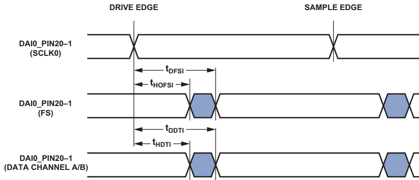
Figure 56. S/PDIF Receiver Internal Digital PLL Mode Timing
