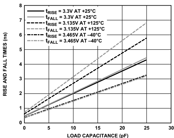
Figure 76. Driver Type A Rise and Fall Times (10% to 90%) vs. Load Capacitance for All Pins Operating at Less Than or Equal to 62.5 MHz
