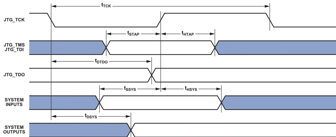
Figure 65. JTAG Port Timing
