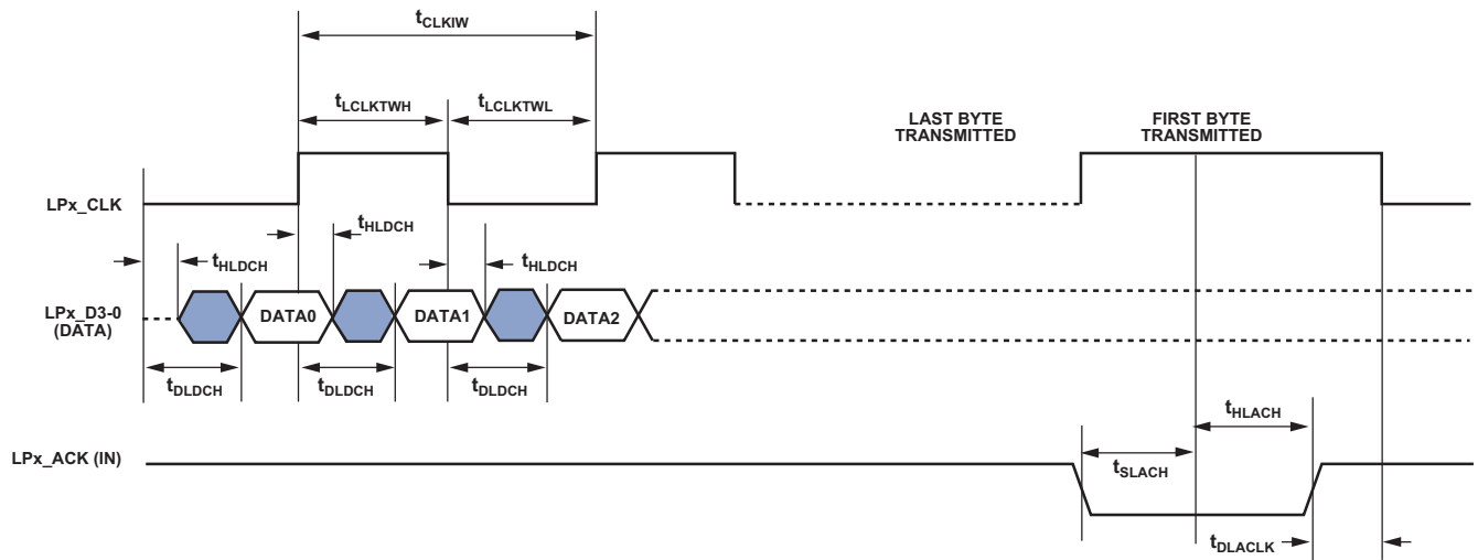
Figure 13. LPs DDR—Transmit
