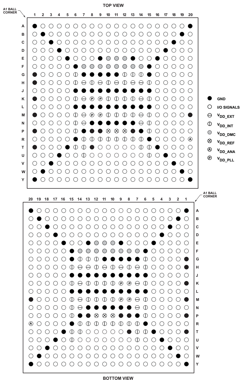
Figure 79. 400-Ball CSP_BGA Configuration
