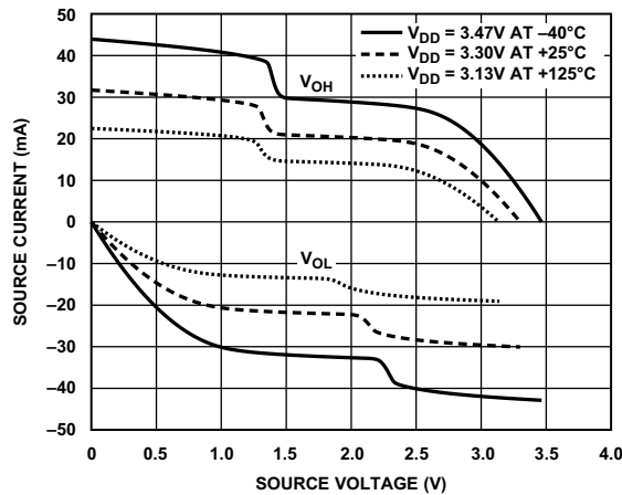
Figure 67. Driver Type A Current for All Pins Operating Above 62.5 MHz and Less Than or Equal to 125 MHz (3.3 V V_{DD\_EXT} )
