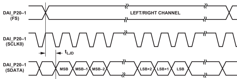
Figure 54. Left Justified Mode
