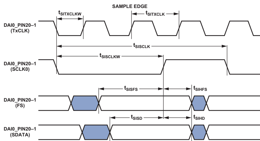
Figure 55. S/PDIF Transmitter Input Timing
