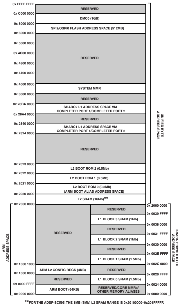
Figure 4. ADSP-SC595/SC596/SC598 Memory Map
