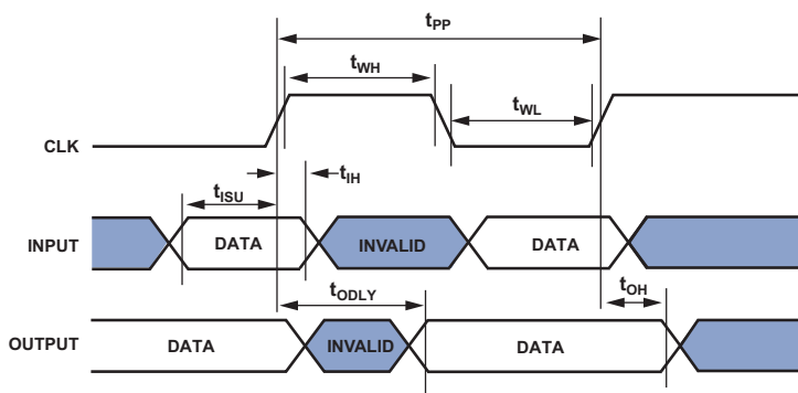
Figure 49. eMSI Controller Timing with eMMC SDR Mode
