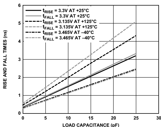
Figure 75. Driver Type A Rise and Fall Times (10% to 90%) vs. Load Capacitance for All Pins Operating Above 62.5 MHz and Less Than or Equal to 125 MHz
