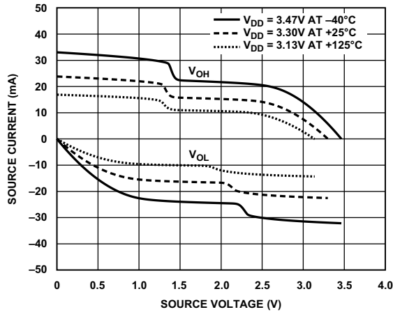
Figure 66. Driver Type A Current for All Pins Operating at Less Than or Equal to 62.5 MHz (3.3 V V_{DD\_EXT} )
