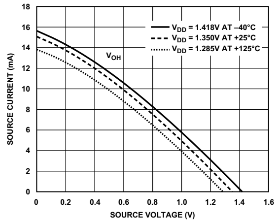
Figure 70. Driver Type B and Driver Type C (DDR3L Drive Strength 100 \Omega )
