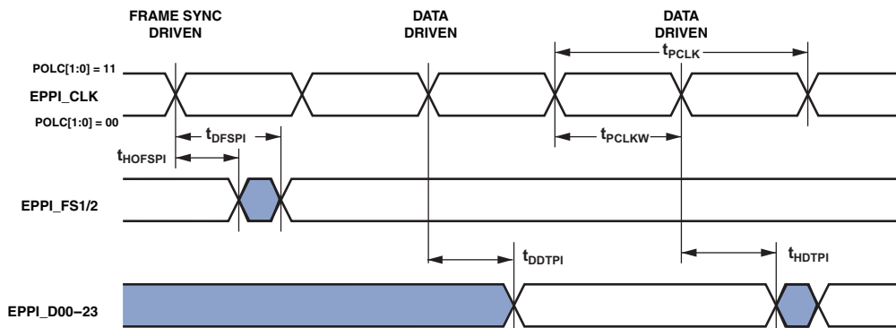
Figure 41. EPPI Internal Clock GP Transmit Mode with Internal Frame Sync Timing
