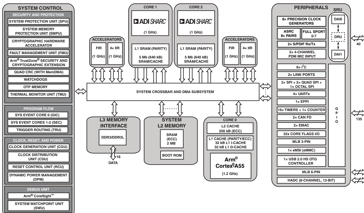
Figure 1. ADSP-SC598 (Full-Featured Model) Processor Block Diagram
