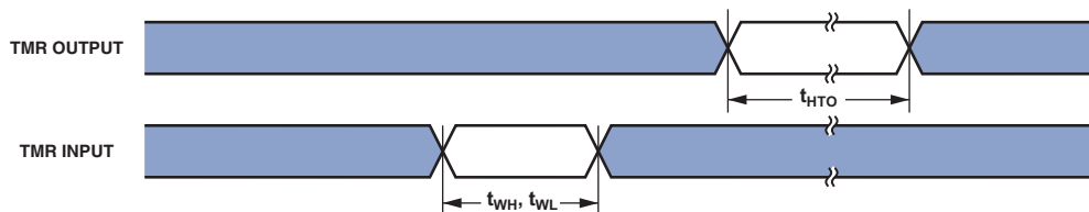
Figure 30. Timer Cycle Timing
