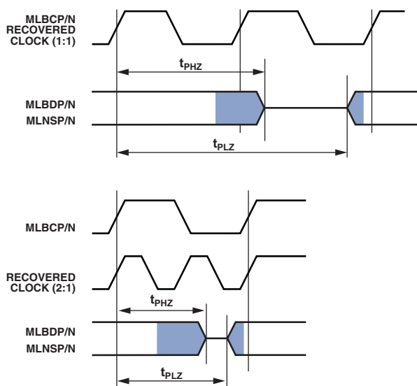
Figure 61. MLB 6-Pin Disable and Enable Turnaround Times
