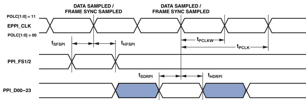
Figure 42. EPPI Internal Clock GP Receive Mode with External Frame Sync Timing
