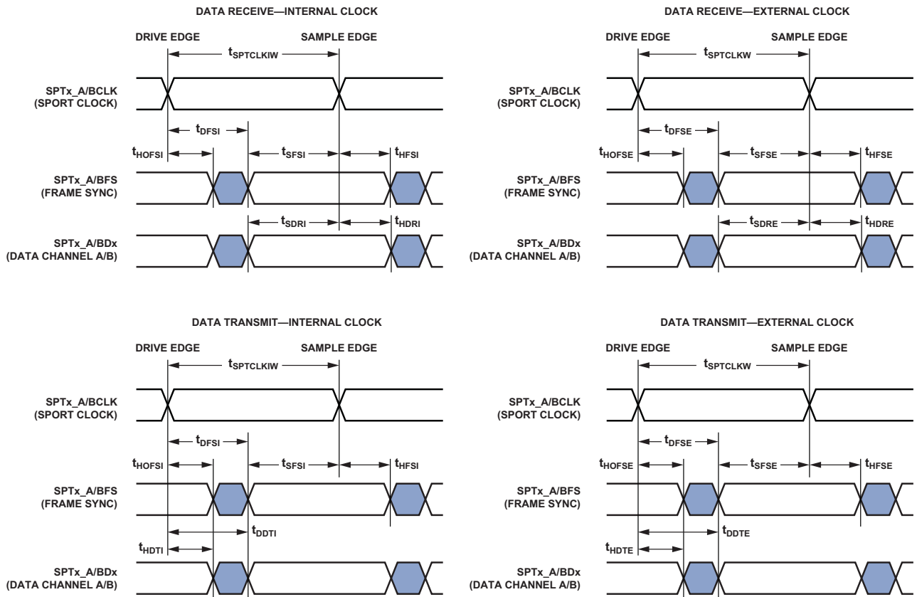
Figure 14. SPORTs
