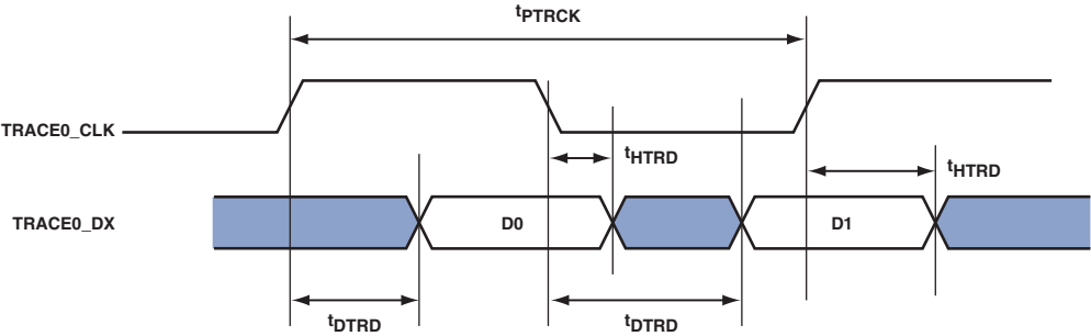
Figure 62. Trace Timing
