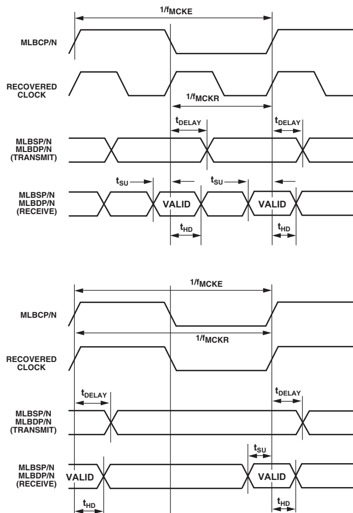
Figure 60. MLB 6-Pin Delay, Setup, and Hold Times
