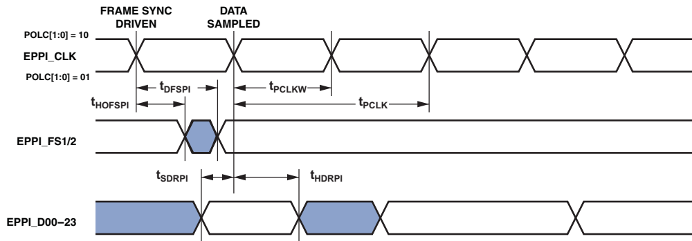
Figure 40. EPPI Internal Clock GP Receive Mode with Internal Frame Sync Timing
