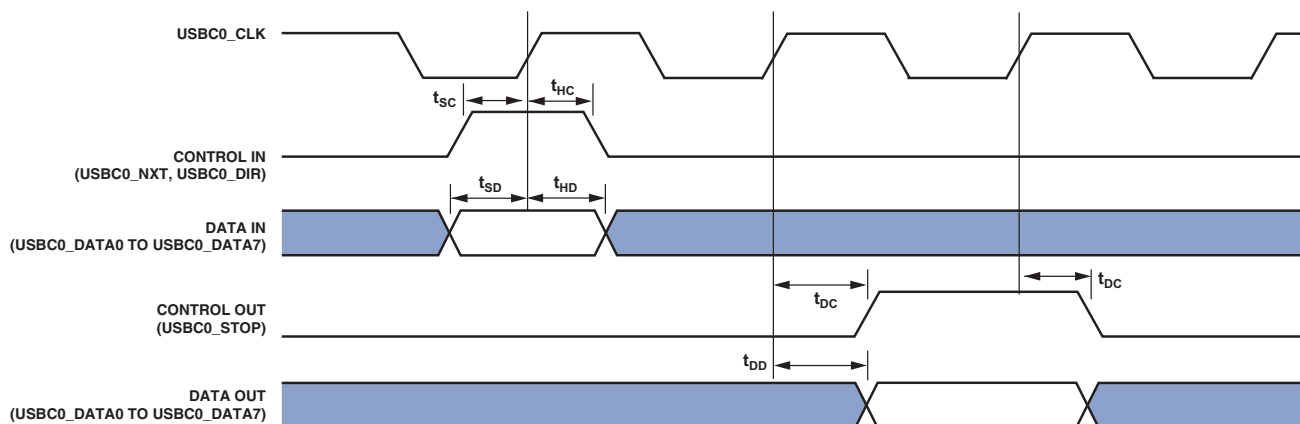
Figure 33. USB Timing
