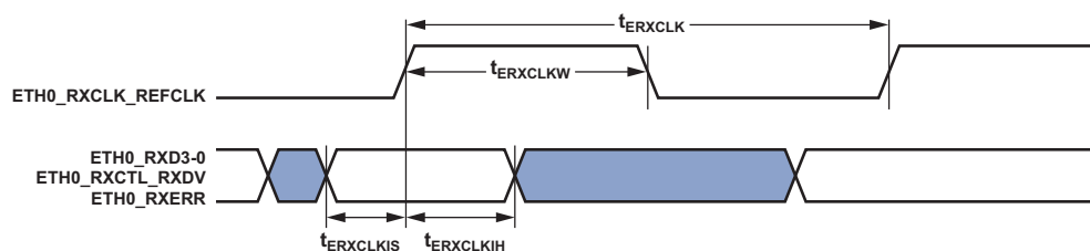
Figure 34. 10/100 EMAC Timing: MII Receive Signal
