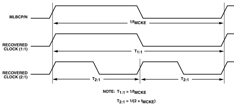
Figure 59. MLB 6-Pin Clock Definitions
