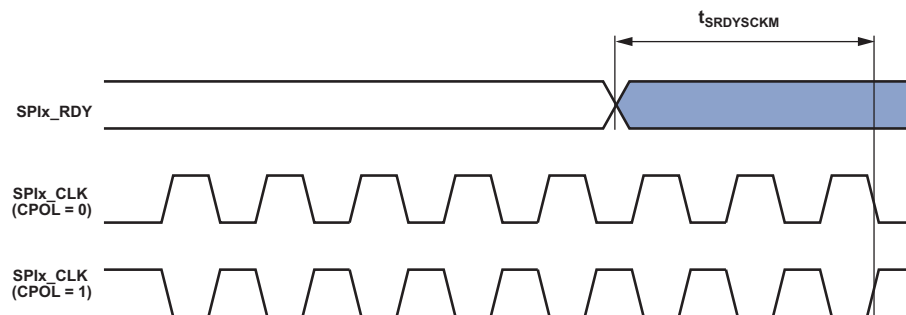
Figure 25. SPIx_RDY Setup Before SPIx_CLK
