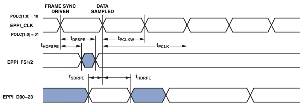
Figure 45. EPPI External Clock GP Receive Mode with Internal Frame Sync Timing
