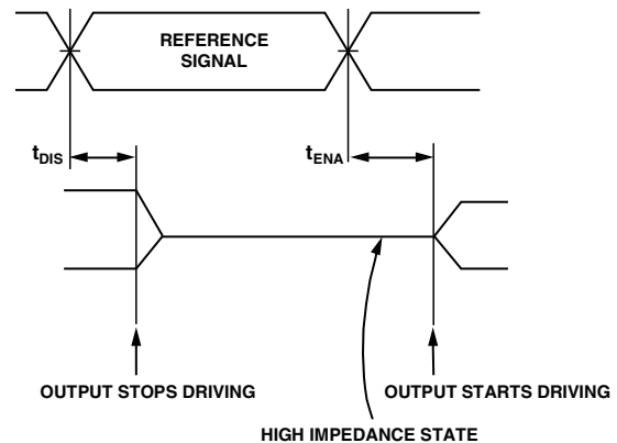
Figure 73. Output Enable/Disable
