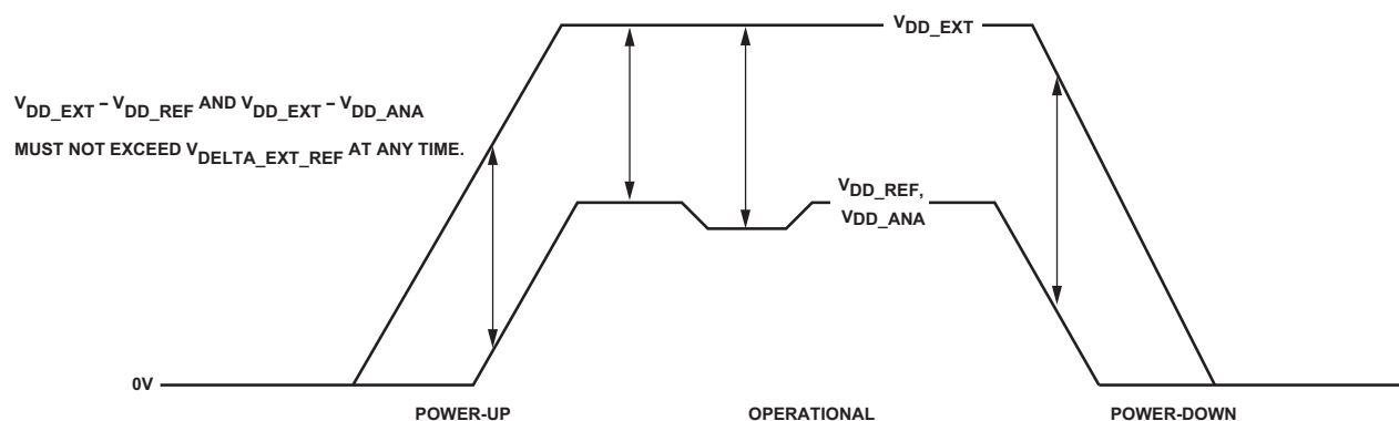
Figure 8. Power-Up and Power-Down Voltage Delta Requirement
