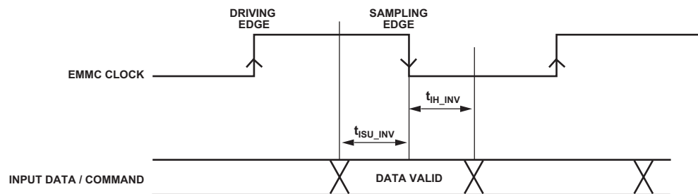
Figure 50. eMSI Controller Timing with eMMC SDR Mode (Clock Tunning Logic Enabled)
