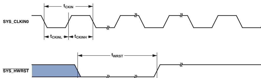
Figure 9. Clock and Reset Timing
