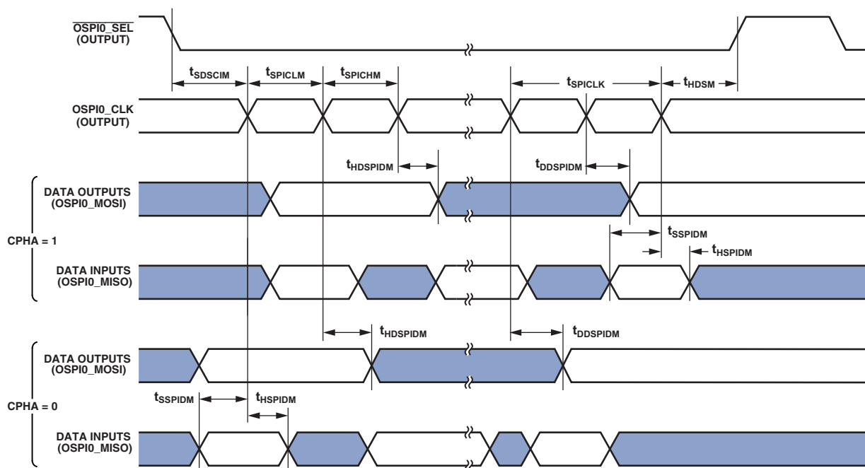
Figure 27. OSPI Port—Master Timing
