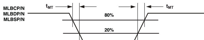
Figure 58. MLB 6-Pin Transition Time
