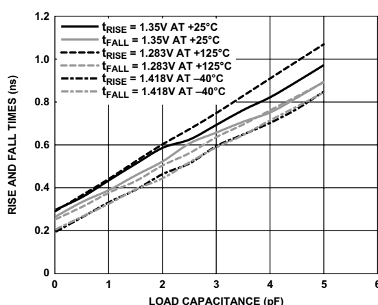
Figure 78. Driver Type B and Driver Type C Rise and Fall Times (10% to 90%) vs. Load Capacitance for DDR3L at 100 Ω
