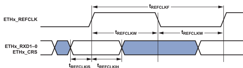
Figure 36. 10/100 EMAC Controller Timing—RMII Receive Signal
