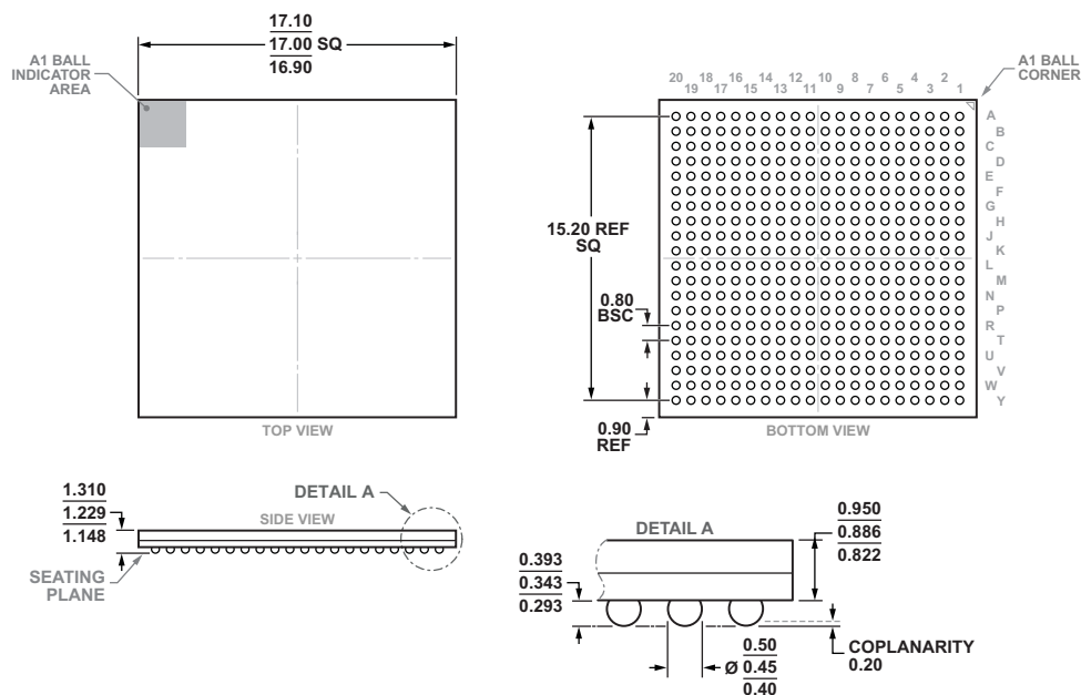
Figure 80. 400-Ball Chip Scale Package Ball Grid Array [CSP_BGA] (BC-400-4) Dimensions shown in millimeters
