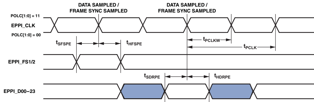
Figure 47. EPPI External Clock GP Receive Mode with External Frame Sync Timing
