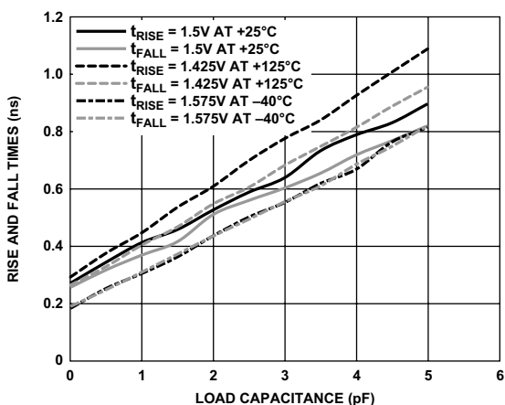
Figure 77. Driver Type B and Driver Type C Typical Rise and Fall Times (10% to 90%) vs. Load Capacitance for DDR3 at 100 Ω
