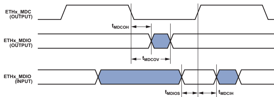
Figure 38. Ethernet MAC Controller Timing— Station Management
