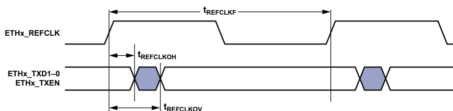
Figure 37. 10/100 EMAC Controller Timing—RMII Transmit Signal
