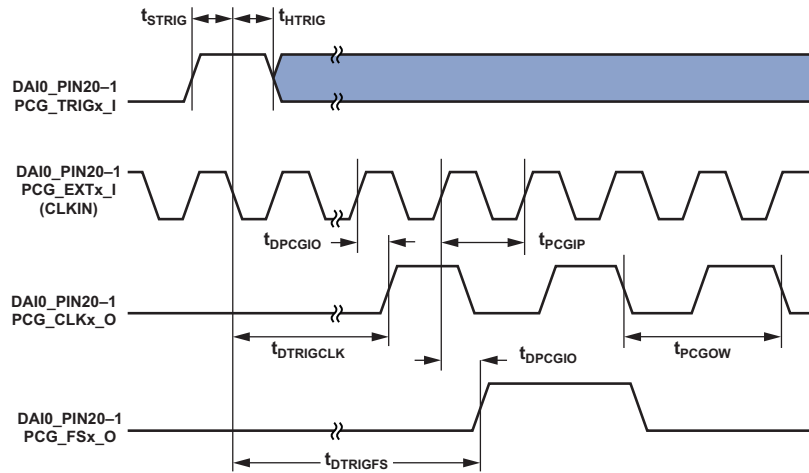
Figure 28. PCG (Direct Pin Routing)
