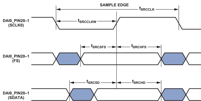
Figure 18. ASRC Serial Input Port Timing
