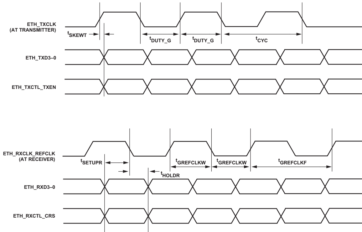
Figure 39. Gigabit EMAC Controller Timing—RGMII
