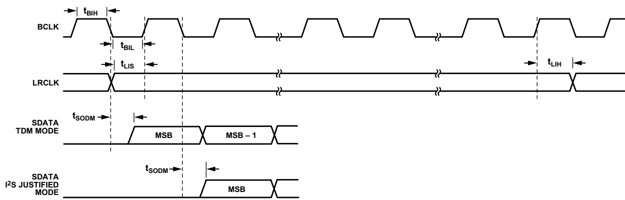
Figure 63. Serial Port Timing
