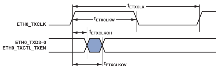
Figure 35. 10/100 EMAC Timing: MII Transmit Signal
