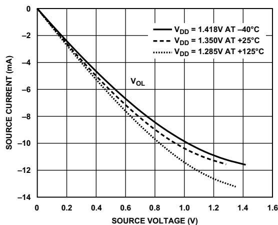
Figure 71. Driver Type B and Driver Type C (DDR3L Drive Strength 100 \Omega )
