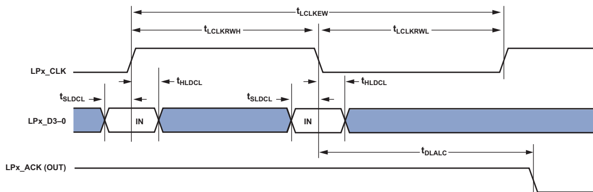
Figure 12. LPs DDR—Receive
