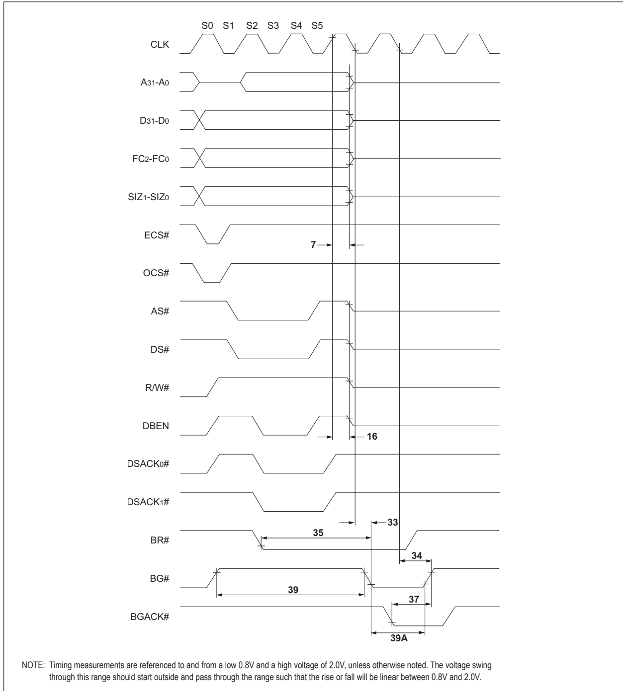
FIGURE 8 – BUS ARBITRATION TIMING DIAGRAM
