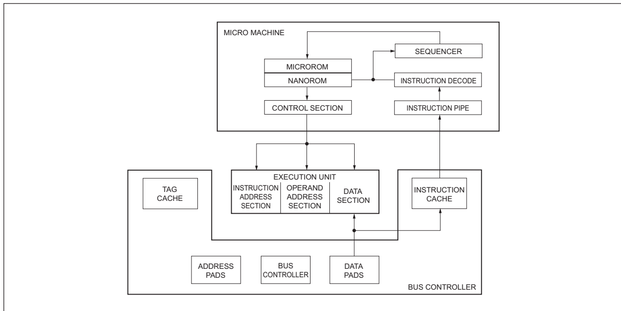
FIGURE 1 – BLOCK DIAGRAM
