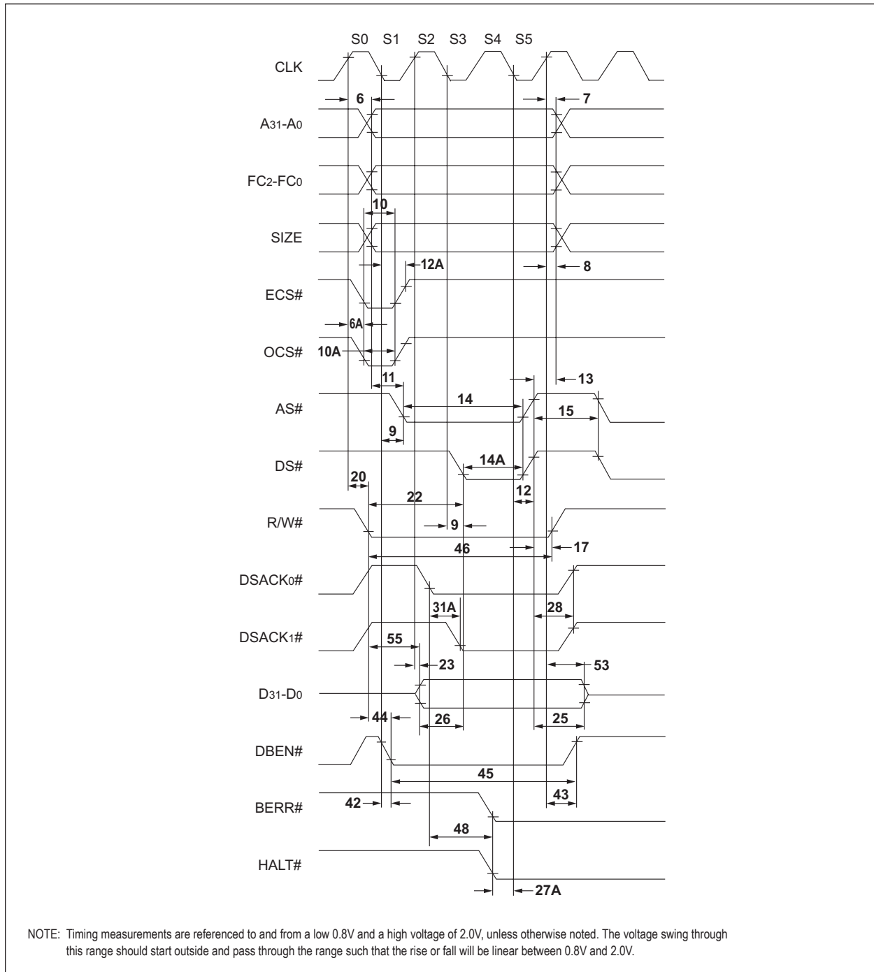
FIGURE 7 – WRITE CYCLE TIMING DIAGRAM
