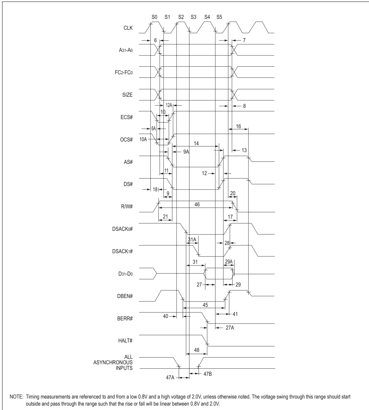
FIGURE 6 – READ CYCLE TIMING DIAGRAM
