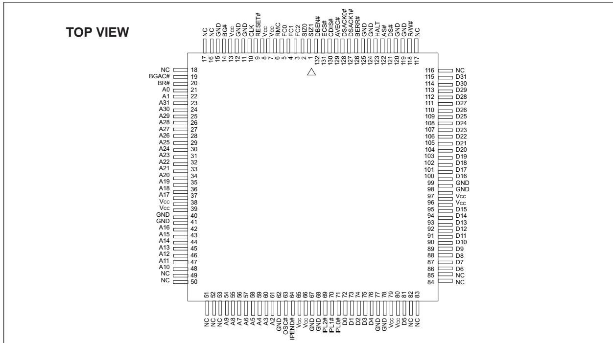
FIGURE 2 – PIN CONFIGURATION FOR WC32P020-XXM, CQFP (Q2)
