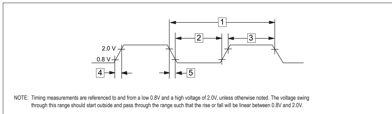
FIGURE 5 – CLOCK INPUT TIMING DIAGRAM
