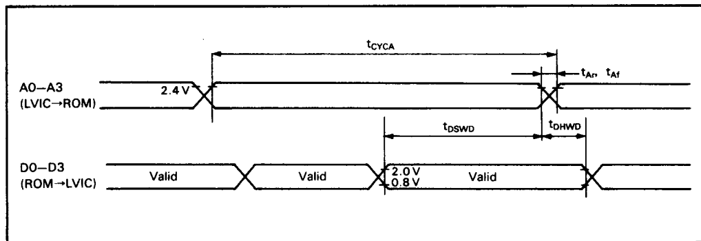
Figure 37 ROM Interface
