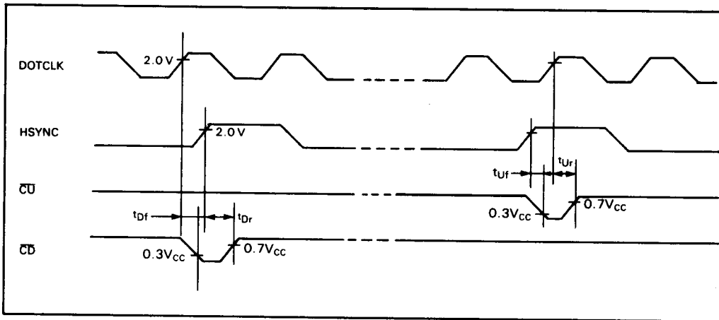
Figure 38 PLL Interface
