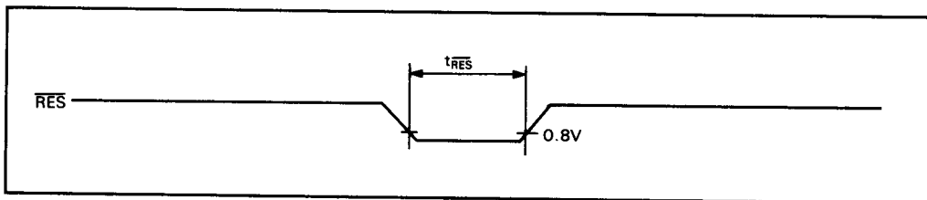
Figure 39 Reset Input
