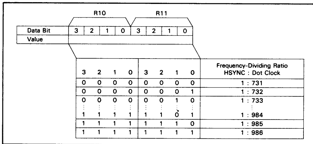
Figure 24 PLL Frequency-Dividing Ratio Register
