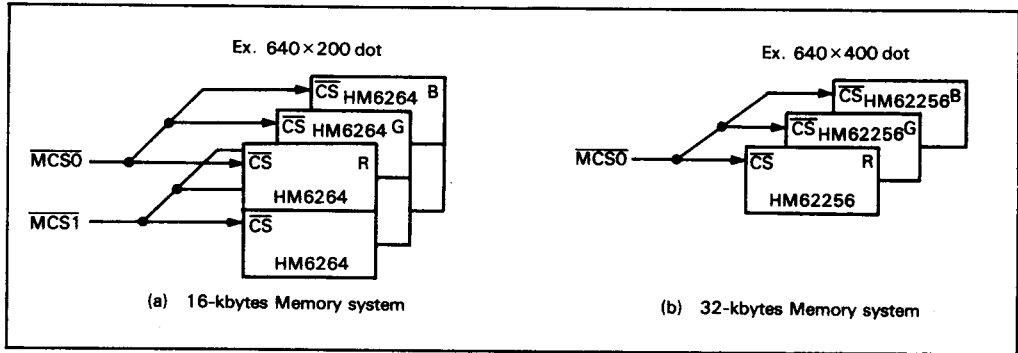
Figure 5 Relation between Display Screen Memories
