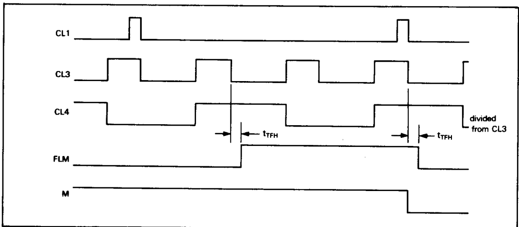
Figure 35 CL1, CL3, CL4, FLM, M (Reduced view of figure 34 in the horizontal stripe mode)
