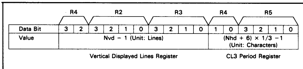
Figure 19 Vertical Displayed Lines Register and CL3 Period Register
