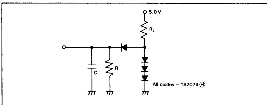
Figure 40 TTL Load Circuit
