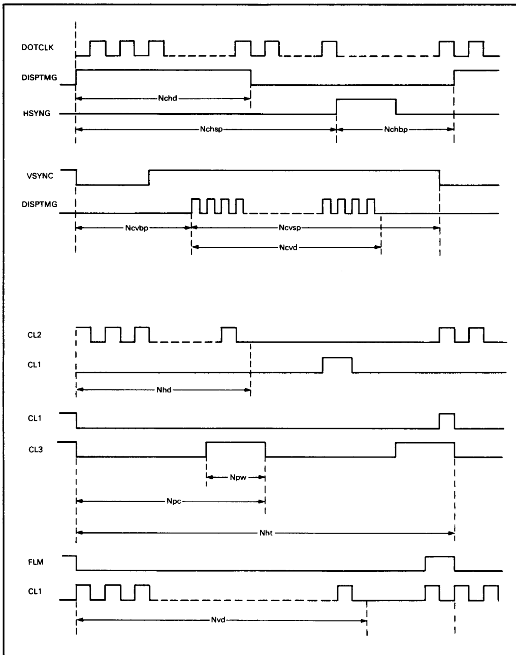
Figure 28 Symbol Definition
