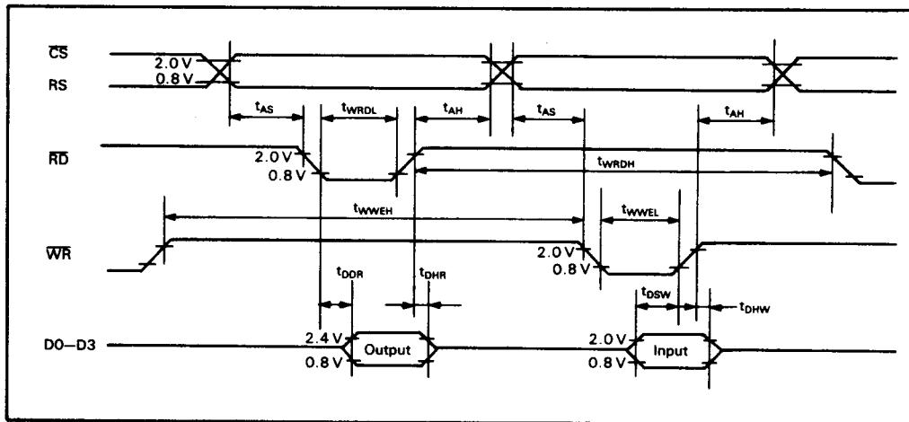
Figure 36 MPU Interface
