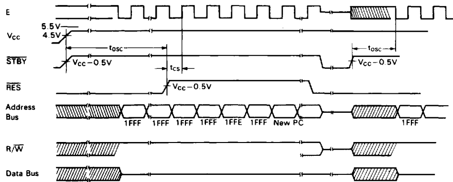
Figure 5 Reset Timing
