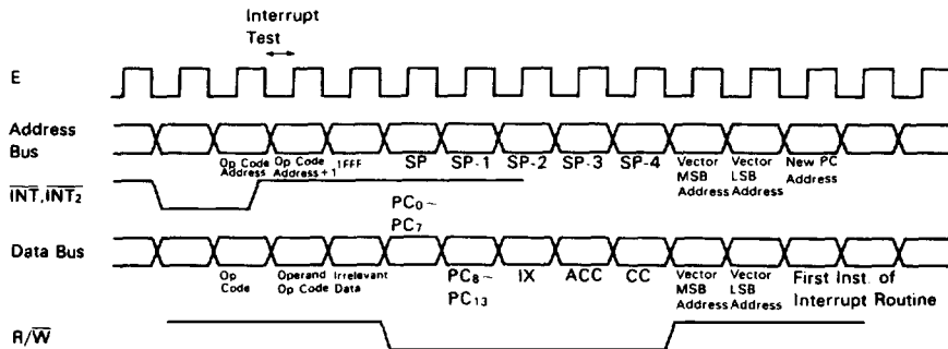
Figure 4 Interrupt Sequence
