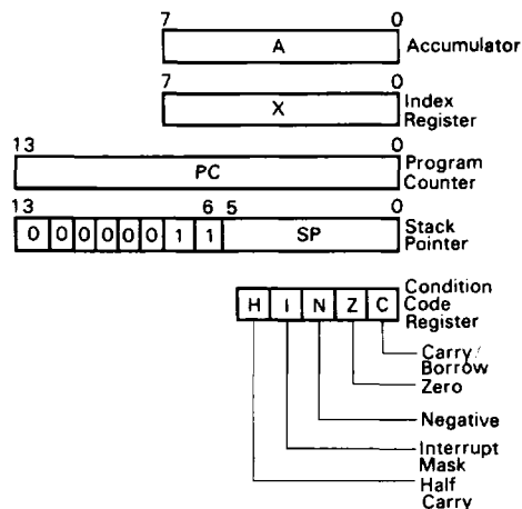
Figure 11 Programming Model
