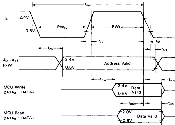
Figure 1 Bus Timing
