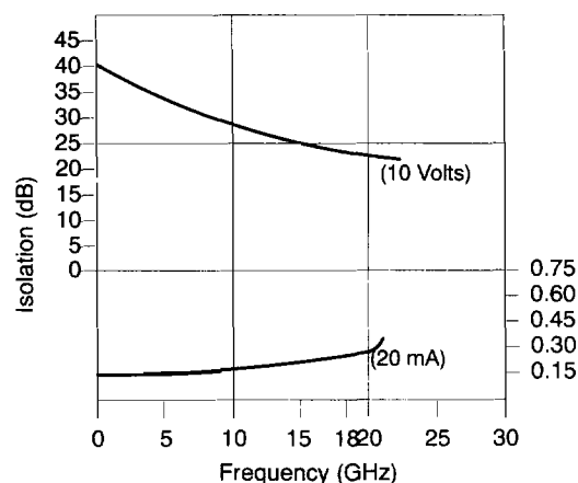
Figure 4. Typical Insertion Loss and Isolation Characteristics
