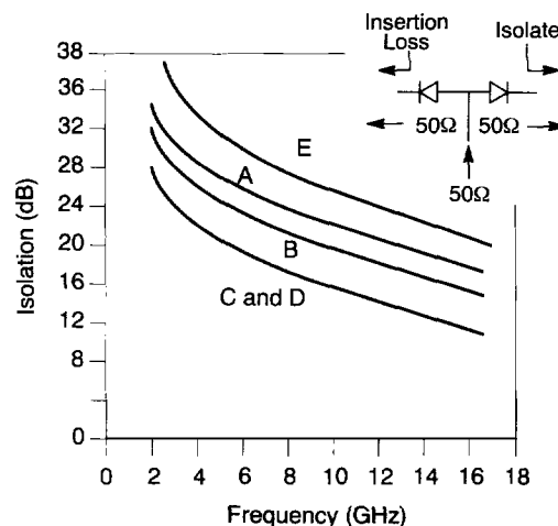
Figure 7. Isolation vs. Frequency, SPDT DSG6470, DSG6474 Series
