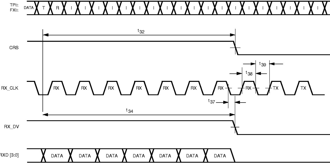
Figure 20. Receive Timing, End of Packet - 100 Mbps
