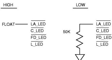
Figure 15. Serial Device Port Address Selection
