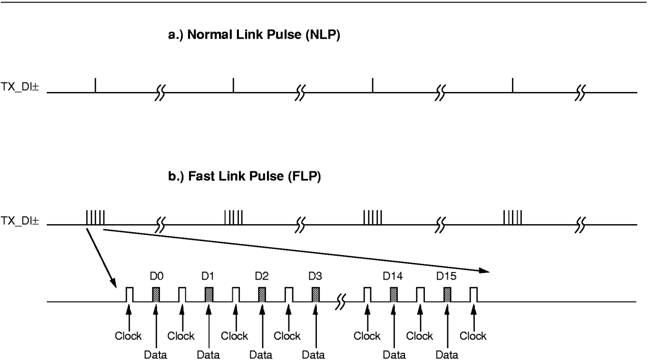
Figure 8. NLP vs. FLP Link Pulse
