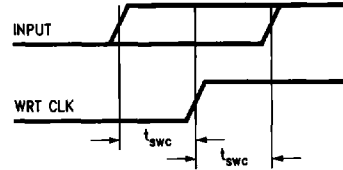
WRT CLK Setup and Hold Times NRZ IN, AME, WRT GATE, READ GATE
