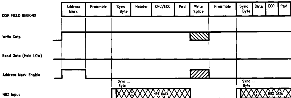
Write Cycle
