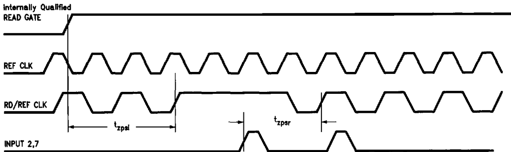
ZPS Stop and Restart Delay Time
