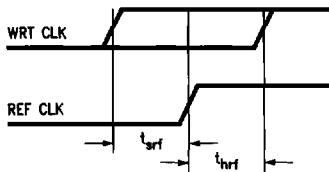
REF CLK Setup and Hold Times
