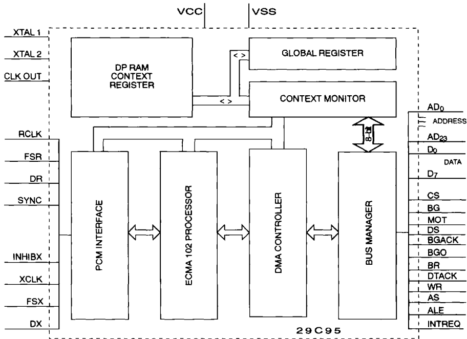
Figure 3. Block Diagram.
