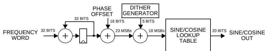
Figure 8. NCO Circuit
