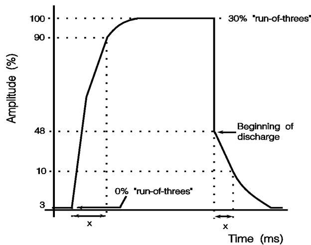
Figure 12: Compand Envelope
