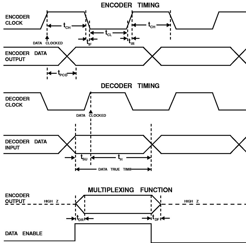
Figure 14: CODEC Timing
