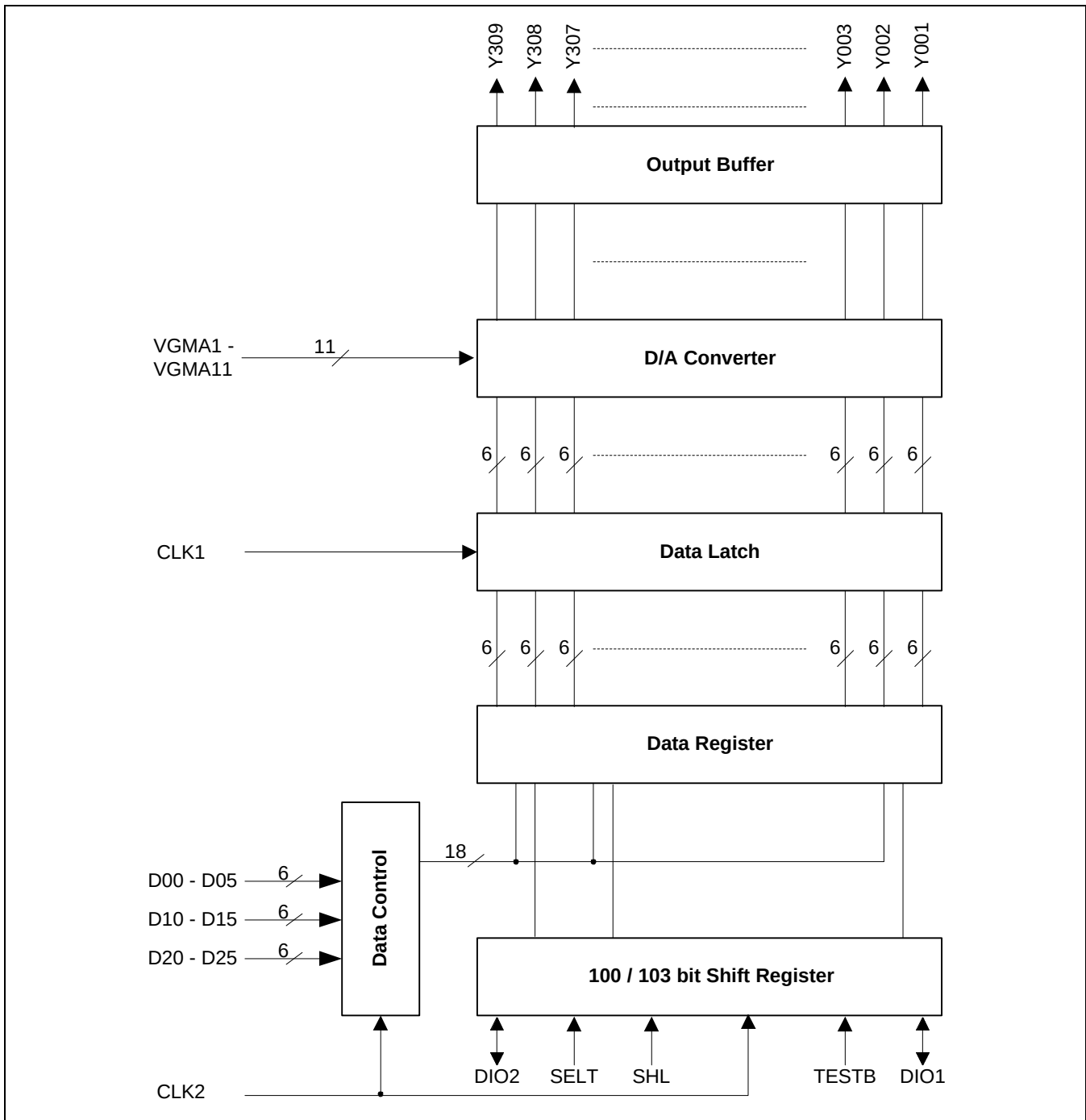
Figure 1. S6C0641 Block Diagram
