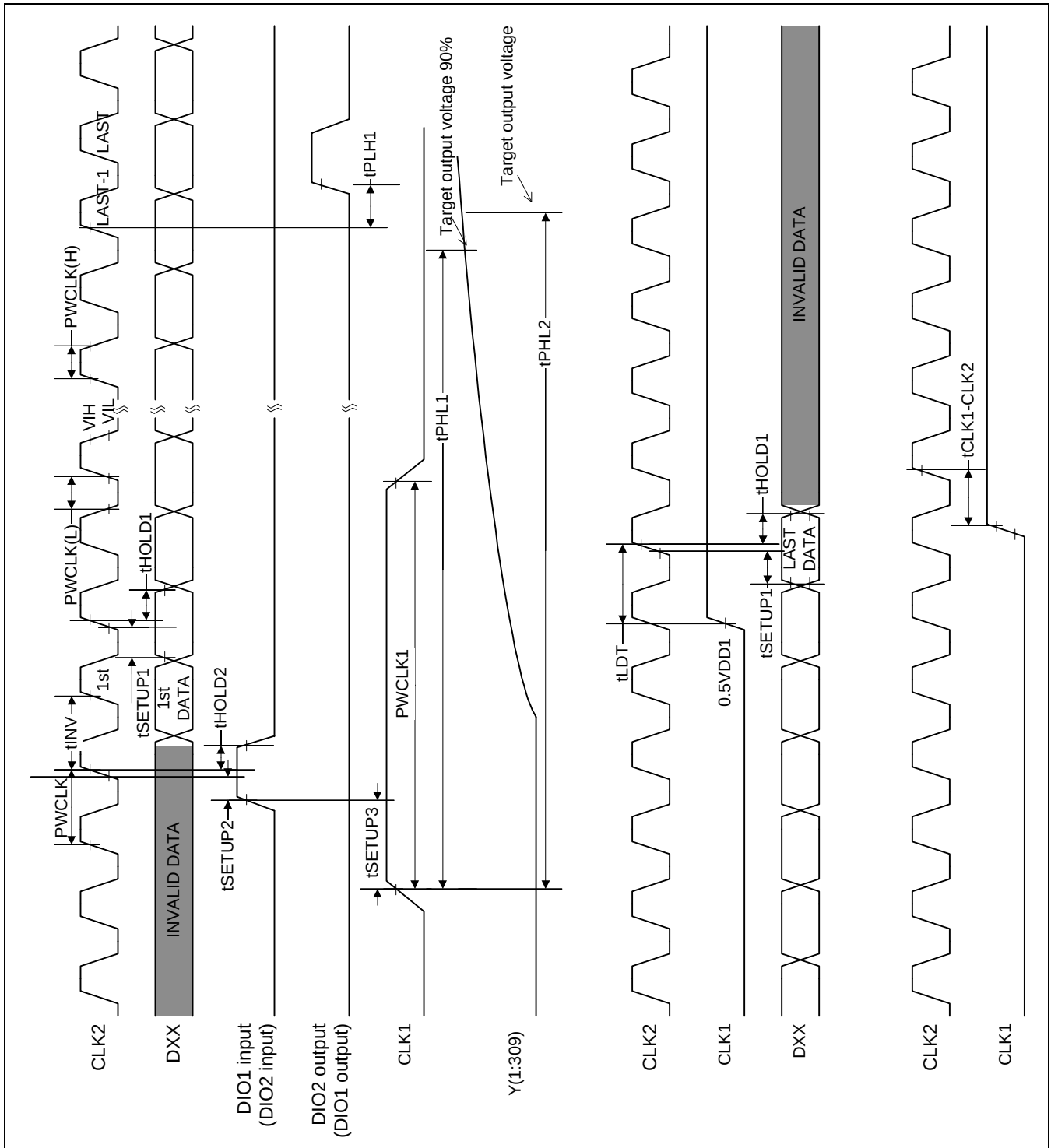
Figure 5. Waveforms
