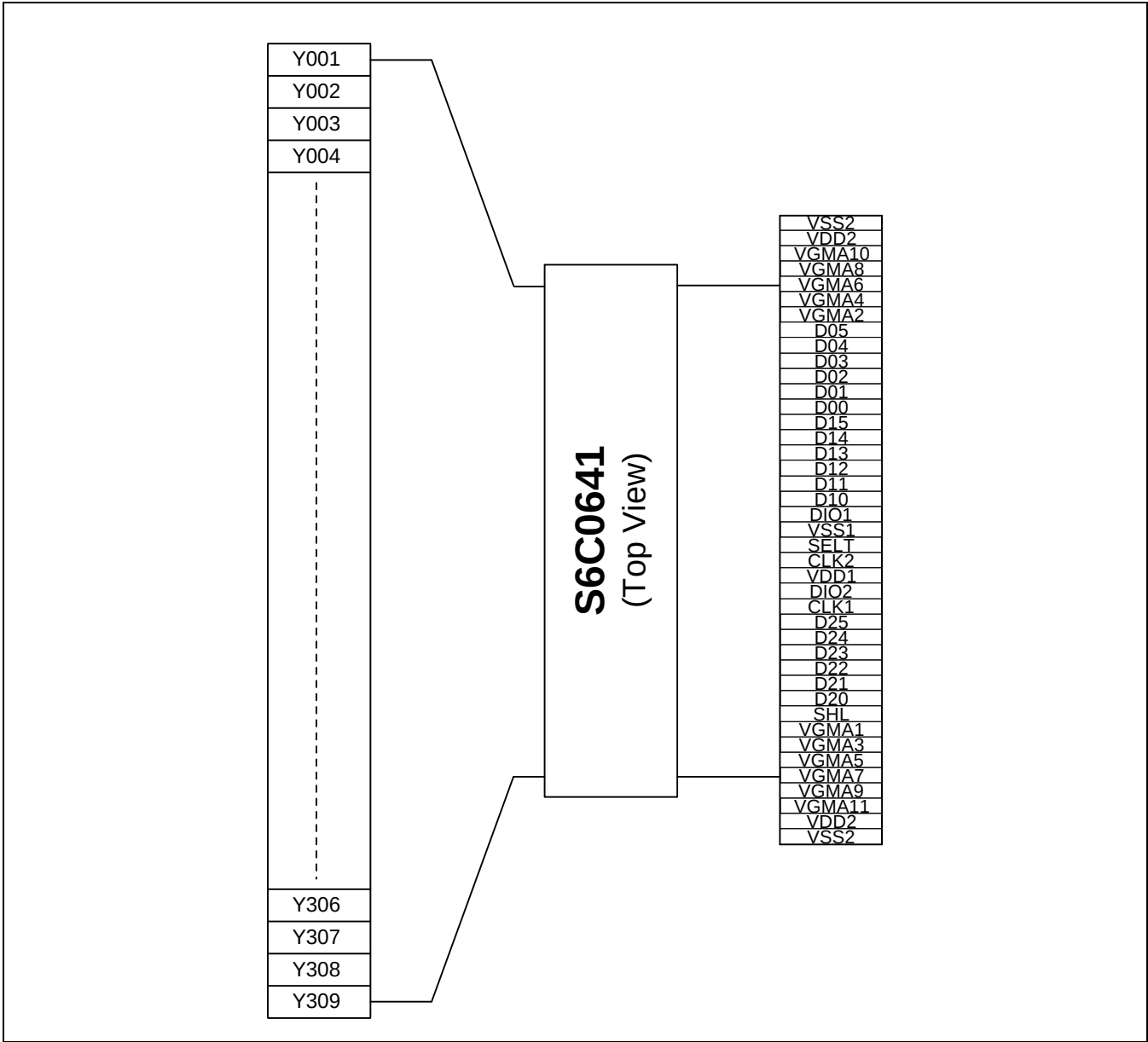
Figure 2. S6C0641 Pin Assignments
