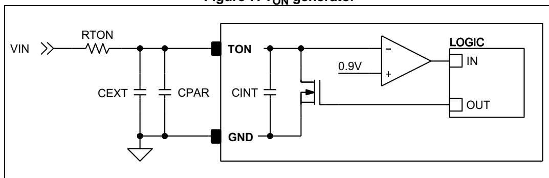
Figure 7. T_{ON} generator
