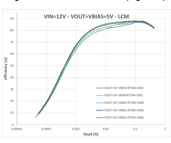
Figure 36. VIN 12 V - VOUT 5 V (log scale)
