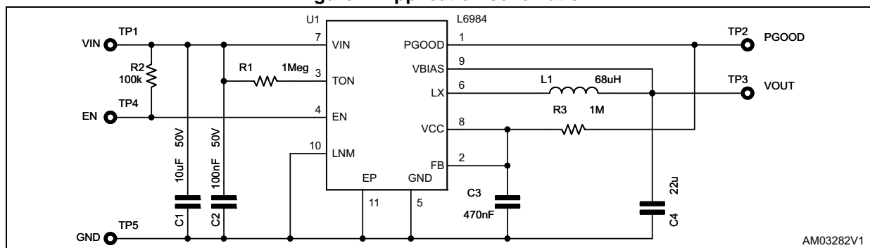
Figure 1. Application schematic
