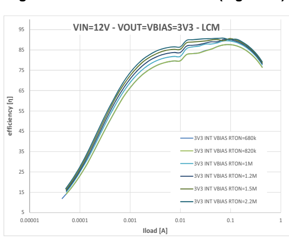
Figure 38. VIN 12 V - VOUT 3.3 V (log scale)
