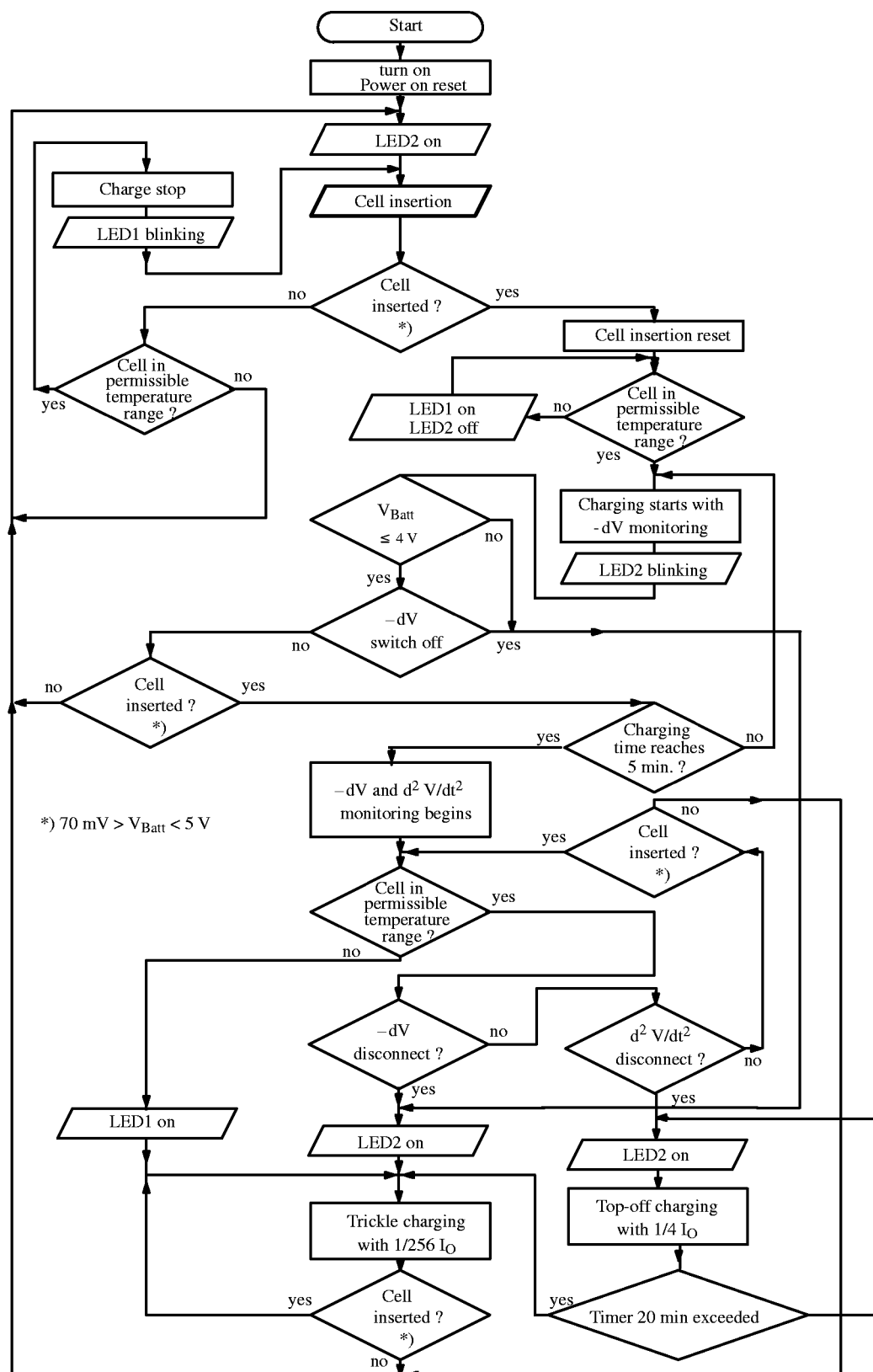
Figure 6. Flow chart
