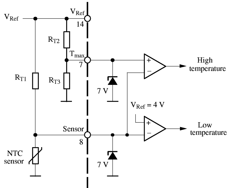
Figure 9. Temperature window
