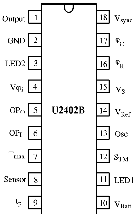
Figure 2. Package: DIP18
