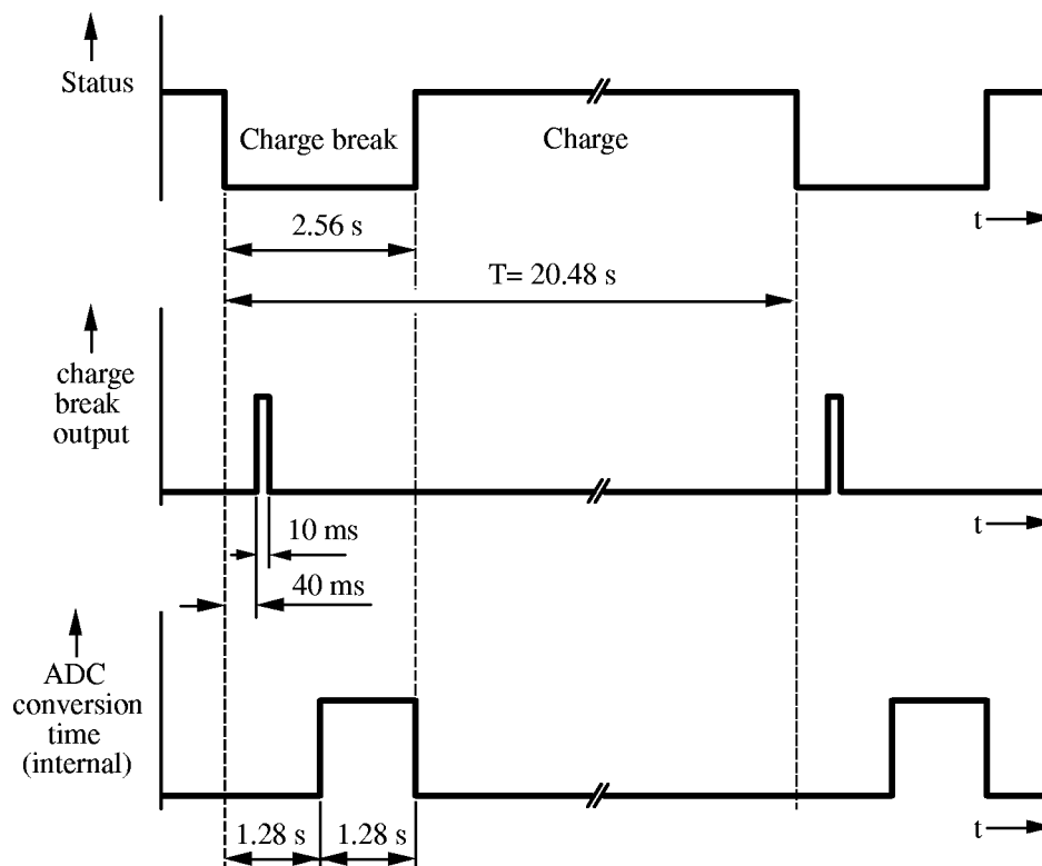
Figure 8. Operating sequence of voltage measurements
