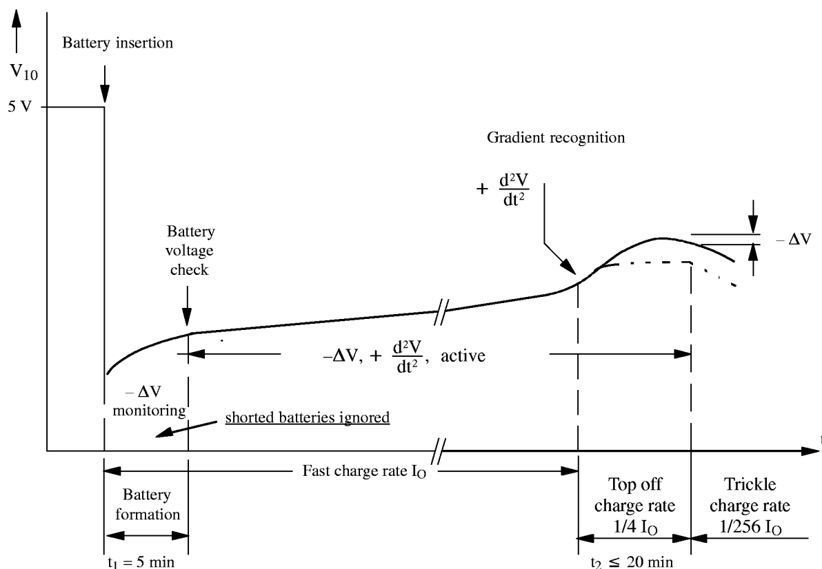
Figure 5. Charge function diagram, f_{osc} = 800 Hz
