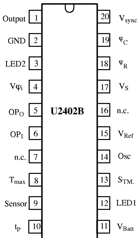
Figure 3. Package: SO20
