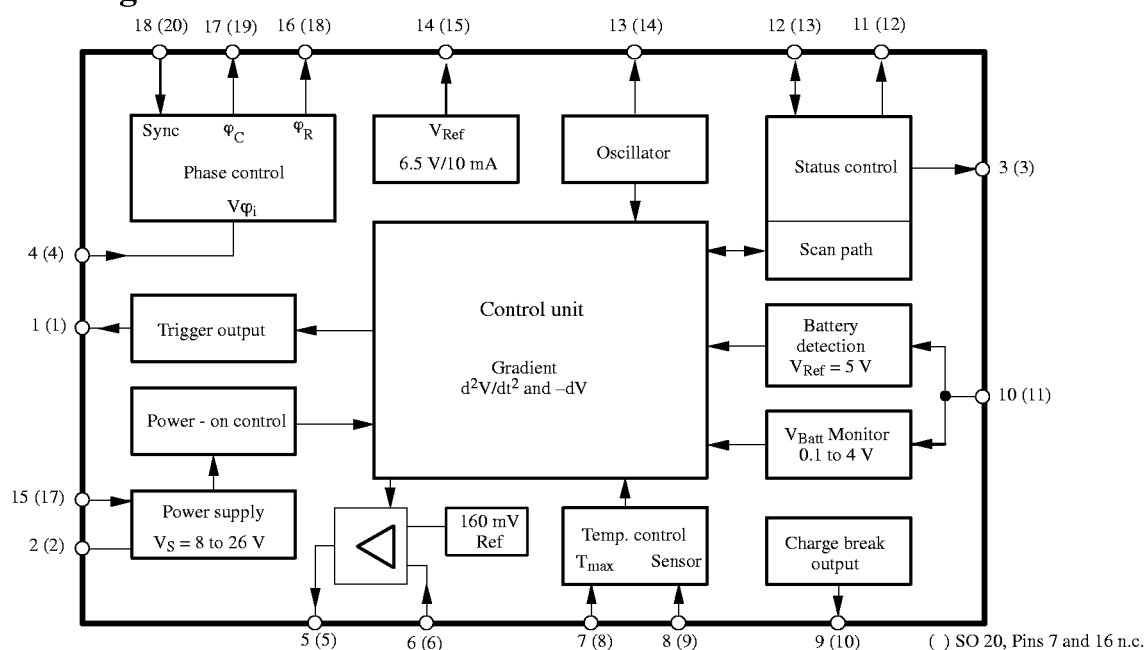
Figure 1. Block diagram
