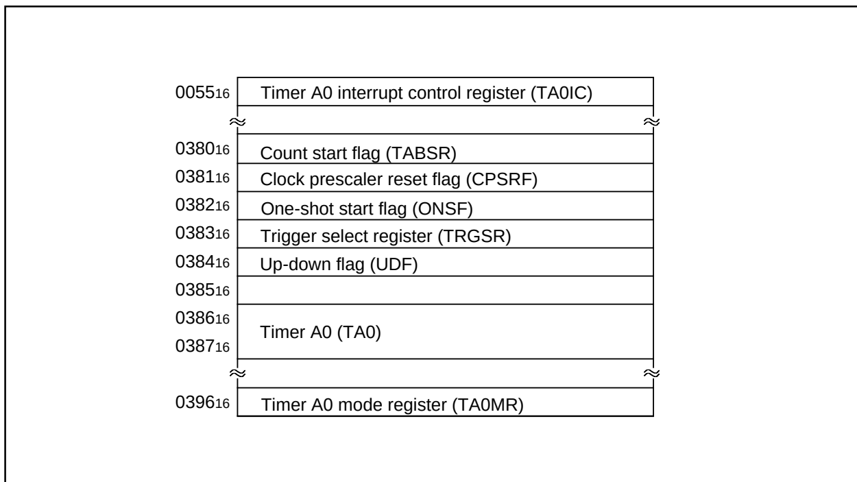
Figure 2.2.1. Memory map of timer A-related registers
