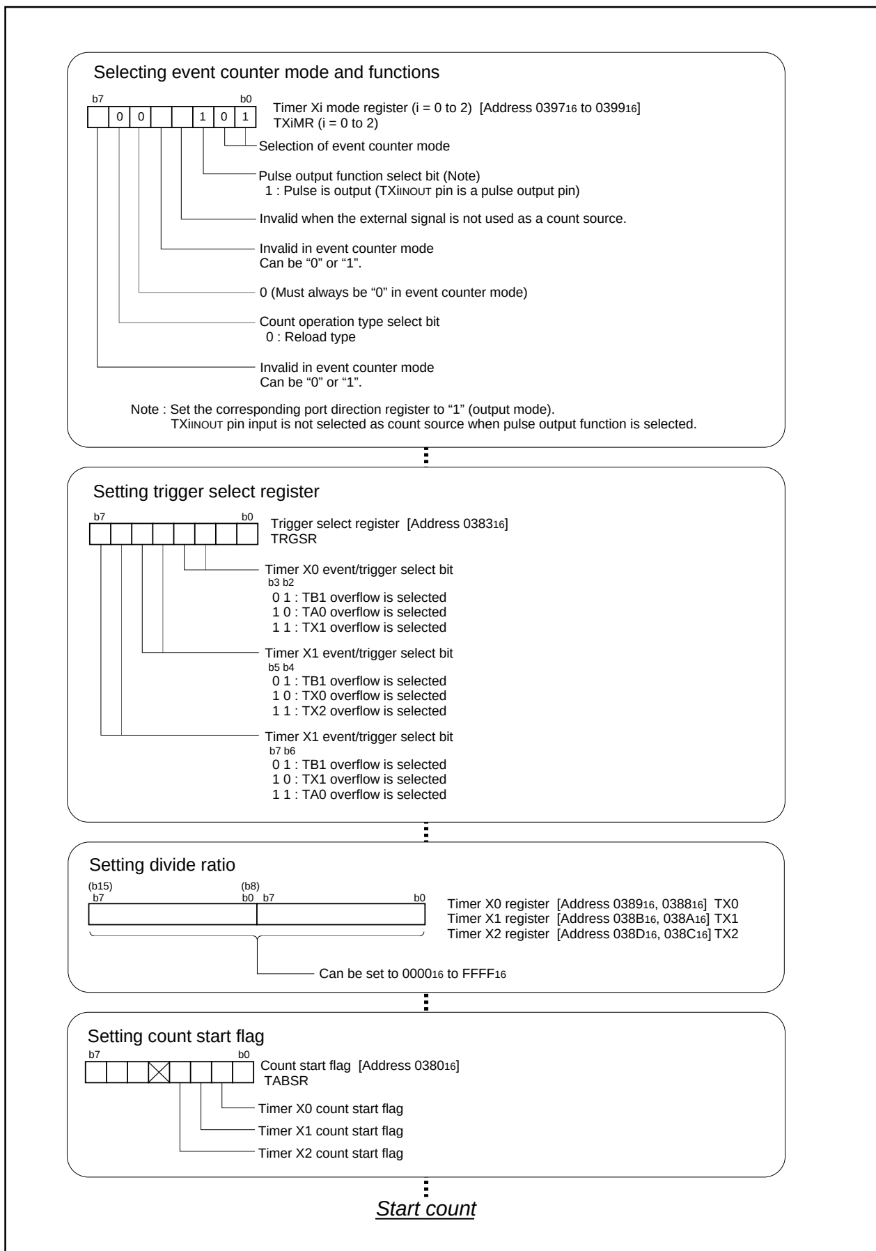
Figure 2.4.11. Set-up procedure of event counter mode, reload type selected
