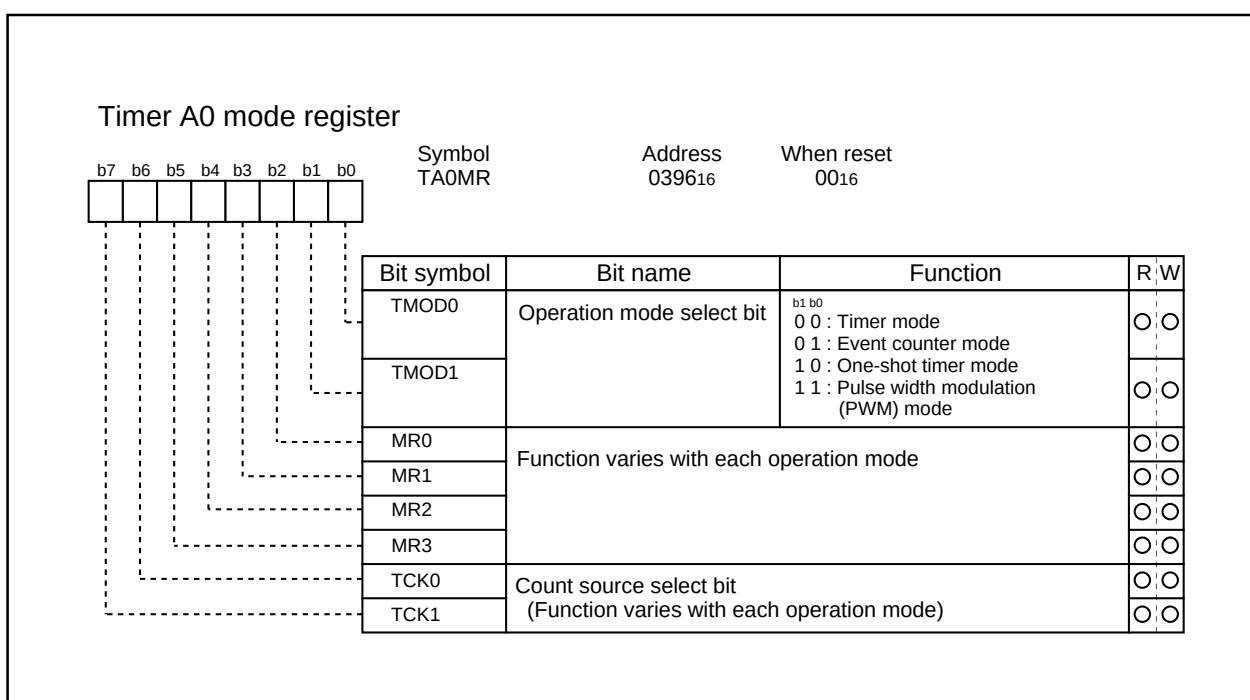
Figure 2.2.2. Timer A-related registers (1)
