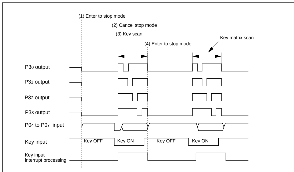
Figure 2.10.4. Example of operation of key-input interrupt
