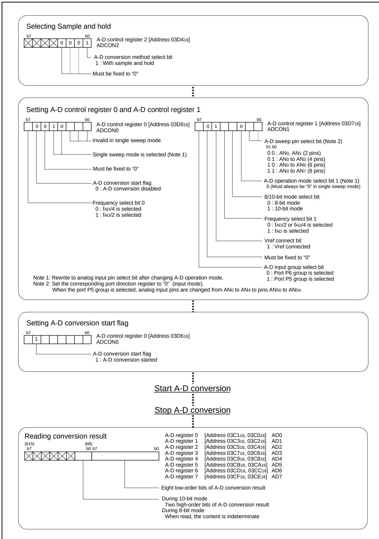
Figure 2.7.10. Set-up procedure of single sweep mode
