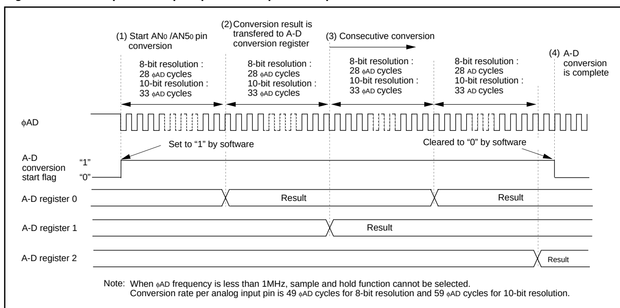
Figure 2.7.14. Operation timing of repeat sweep 1 mode
