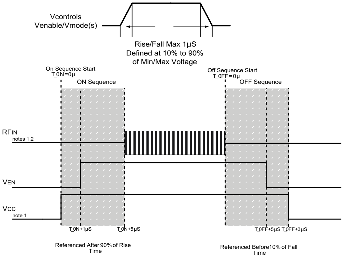
Figure 3: Recommended ON/OFF Timing Sequence
