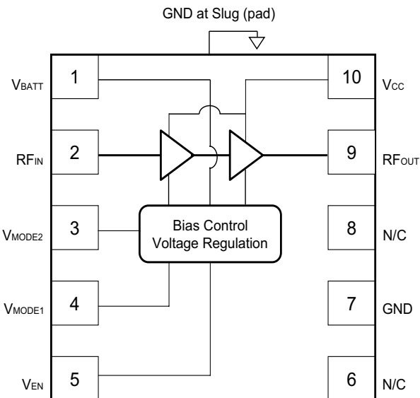
Figure 1: Block Diagram
