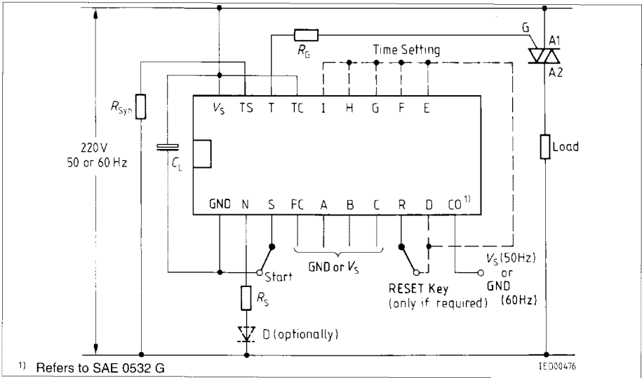
Application Circuit 1 Operation with resistive load
