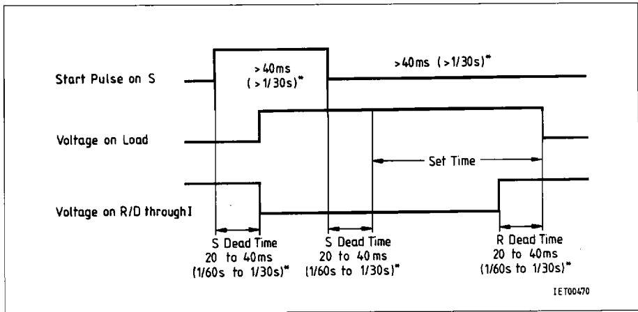
Figure 2 Dropout Delay
