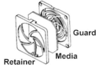
551147 Finger Guard
