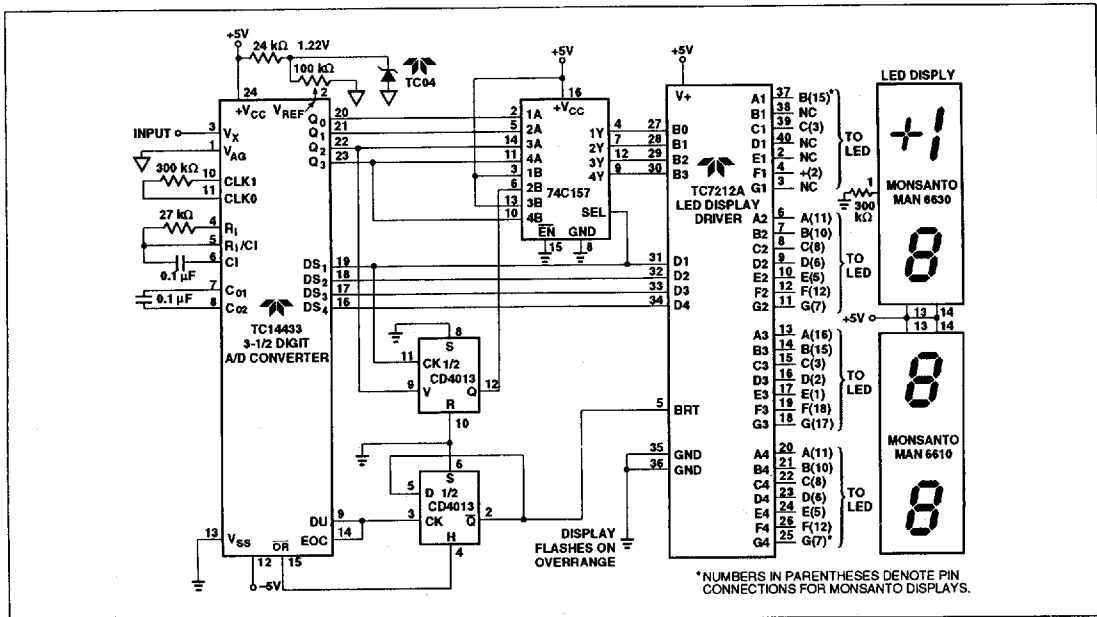
Figure 15. TC7212A Interface to TC14433 3-1/2 Digit ADC
