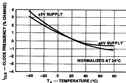
Figure 6. Typical % Change of Clock Frequency vs Temperature
