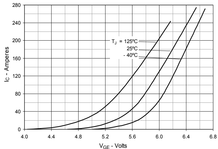
Fig. 5. Input Admittance
