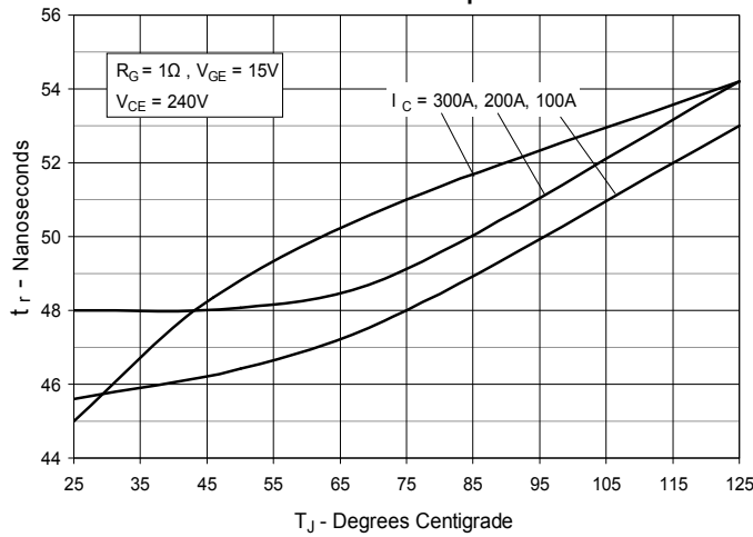
Fig. 11. Resistive Turn-on Rise Time vs. Junction Temperature
