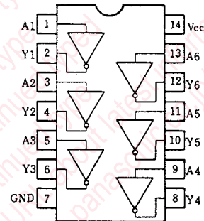
Pin Configuration
