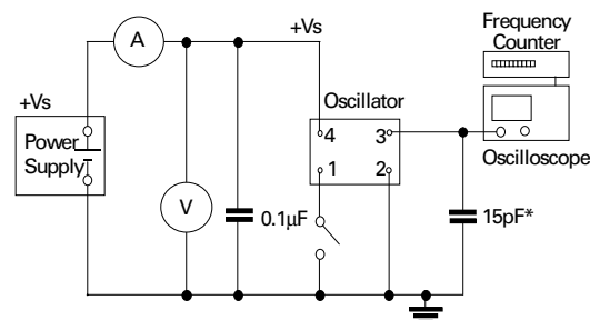
Test Circuit - HCMOS
