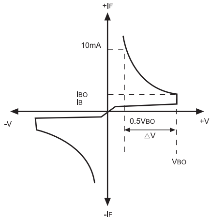
FIG.1 - CURRENT-VOLTAGE CHARACTERISTICS
