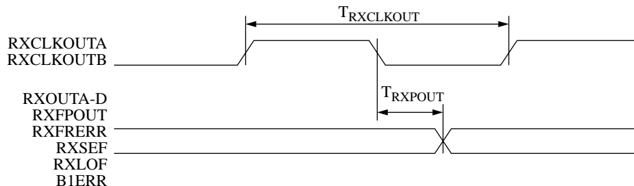
Figure 19: VSC8024 Parallel Data Output Timing Diagram
