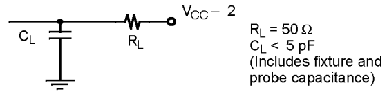
(b) PECL AC Test Load [7]
