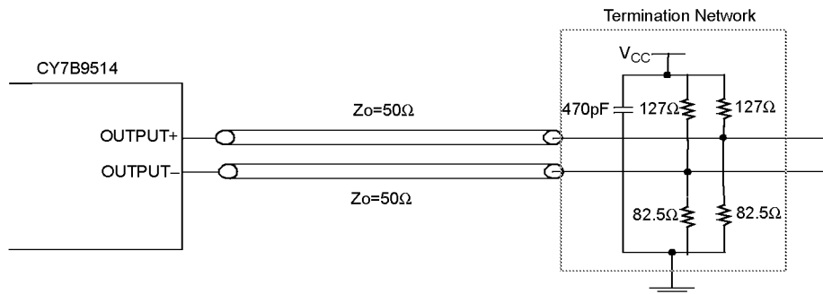
Figure 2. Termination Network Design
