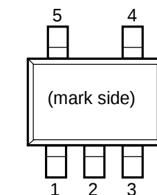
RP118N (SOT-23-5) Pin Configuration
