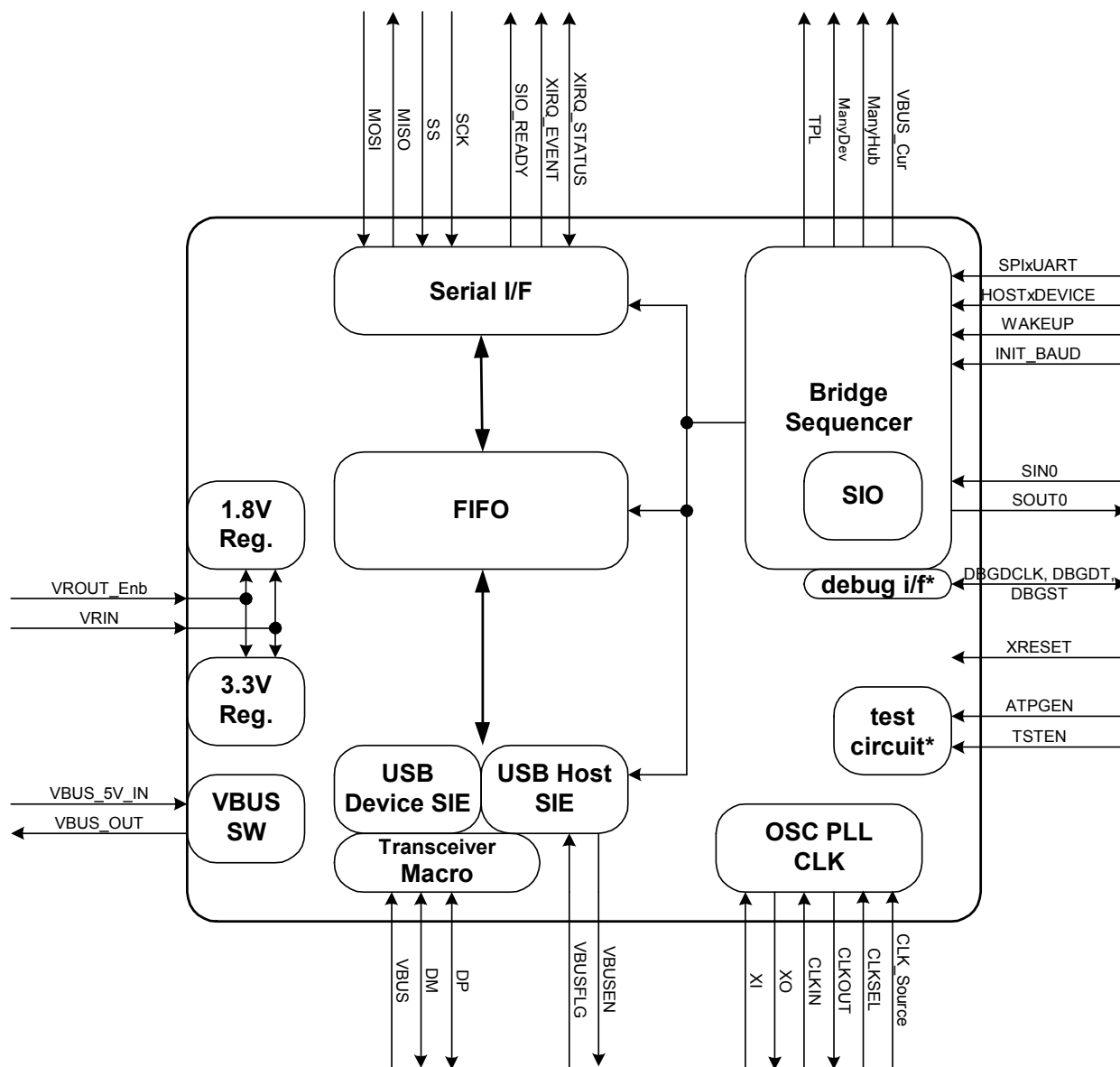
Figure 3.1 Block diagram
