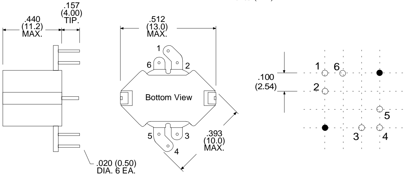
Physical Dimensions inches (mm)
