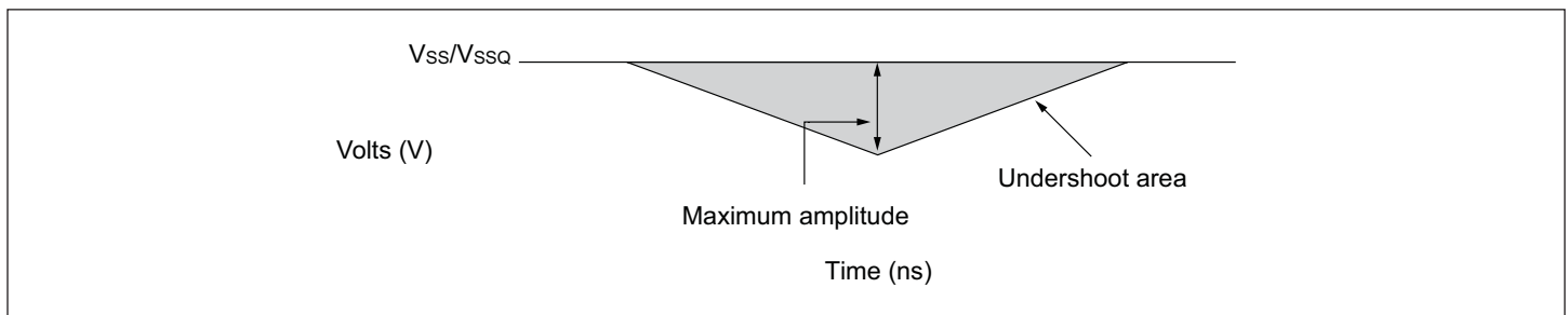
FIGURE 15 – UNDERSHOOT
