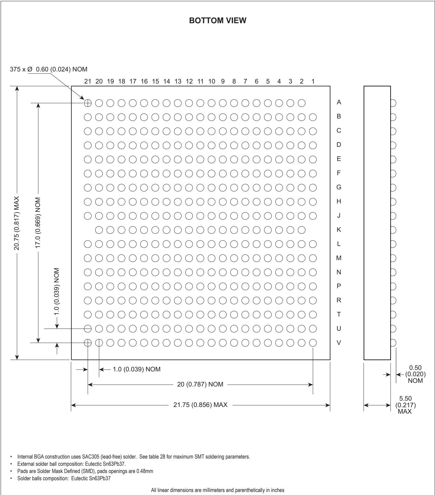
FIGURE 16 – PACKAGE DIMENSION: 375 PLASTIC BALL GRID ARRAY (PBGA) for W3J128M72G-XPBX
