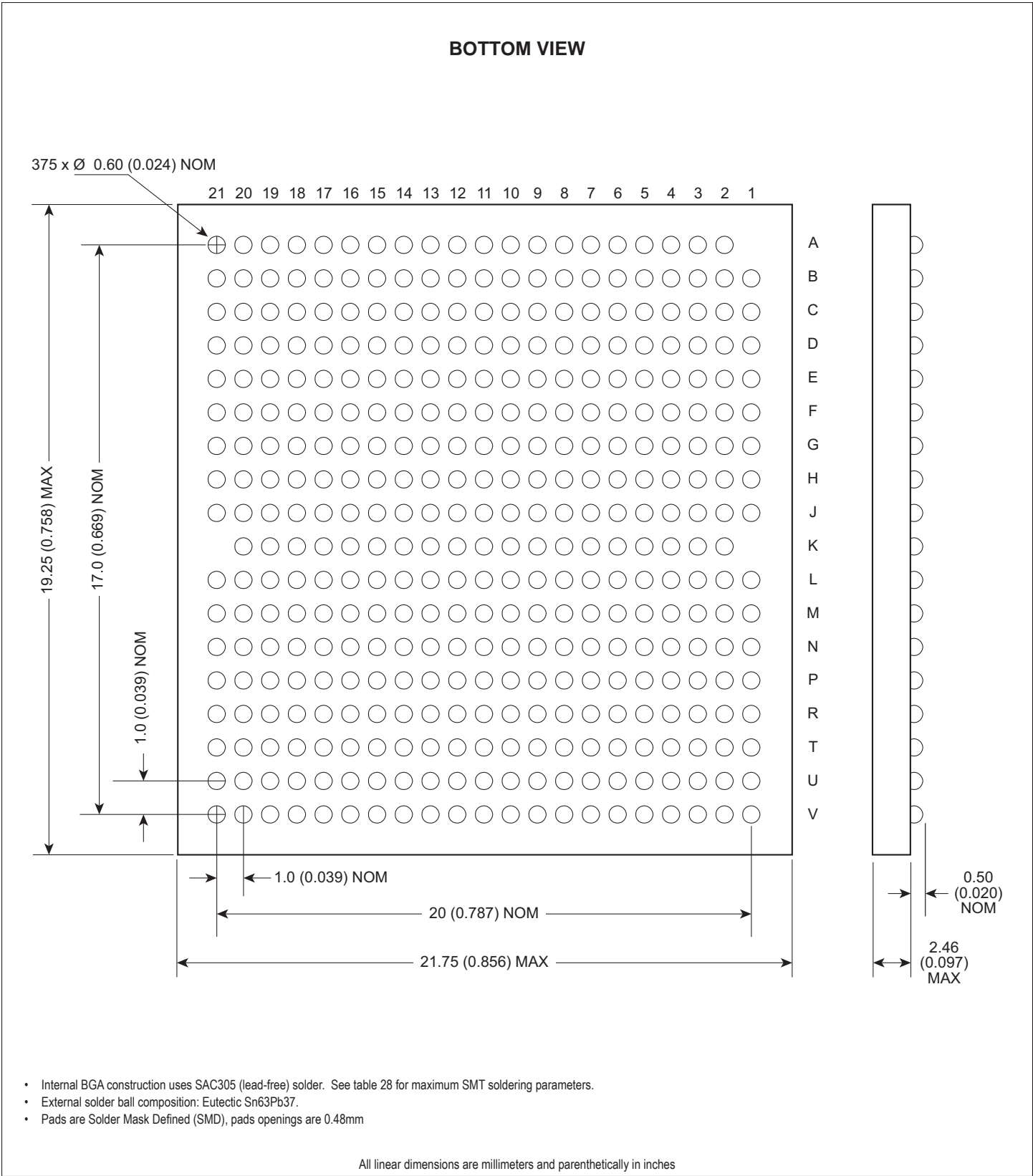
FIGURE 16A – PACKAGE DIMENSION: 375 PLASTIC BALL GRID ARRAY (PBGA) FOR W3J128M72G-XPBX
