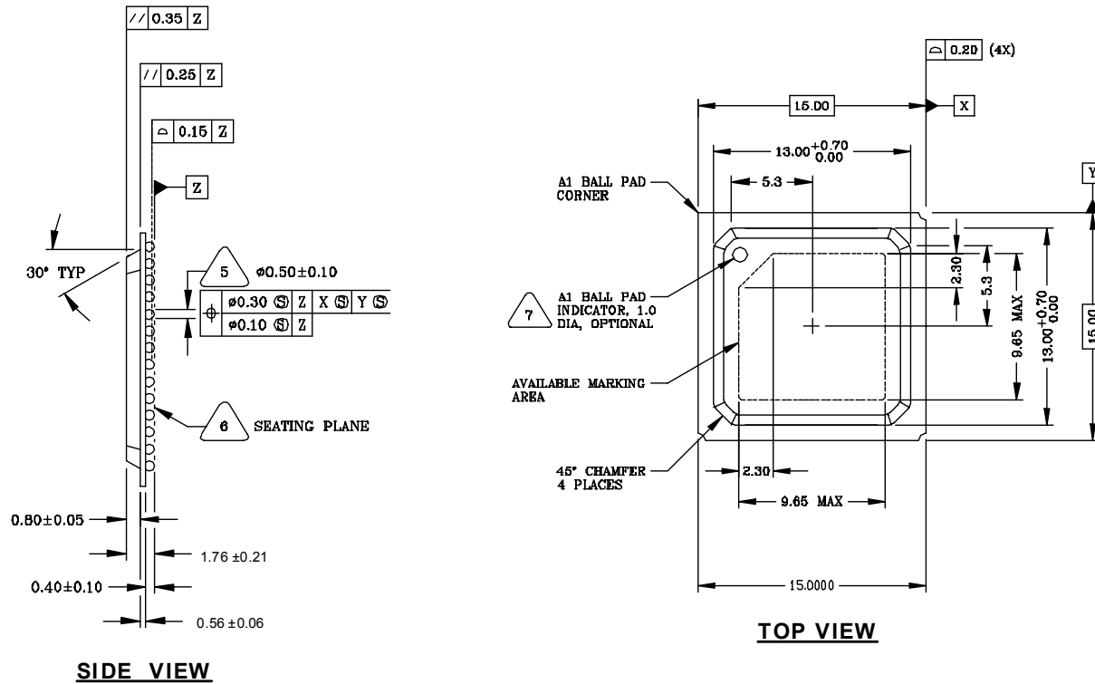
Figure 11. Package Drawing
