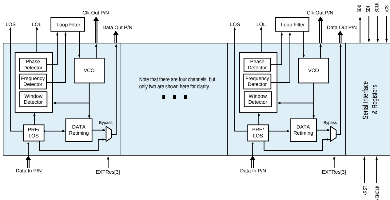
Figure 1. Block Diagram
