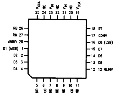
28-Lead Plastic Chip Carrier—V Package
