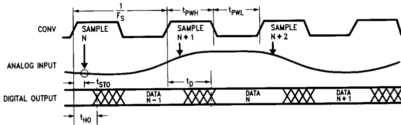
FIGURE 1. Timing Diagram
