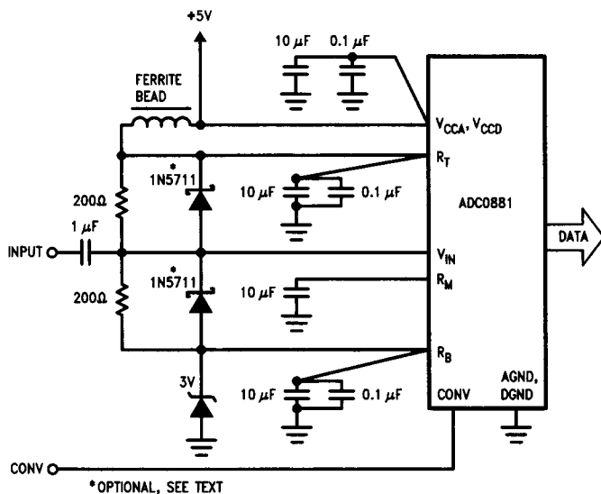
FIGURE 7. Inexpensive Interface Circuit
