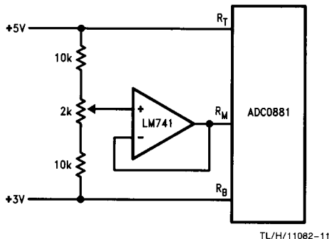
FIGURE 5. Optional Midscale Linearity Adjust
