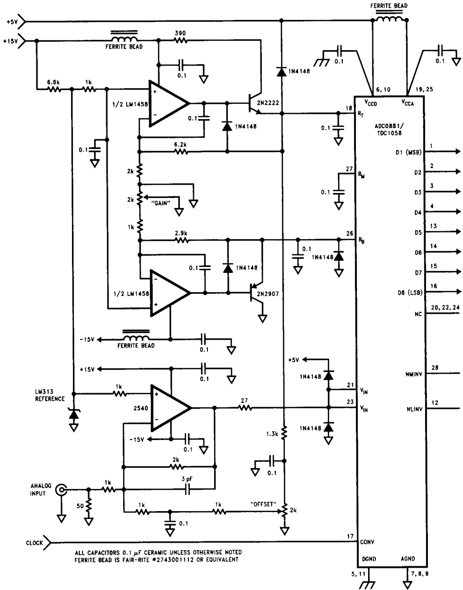
FIGURE 6. Typical Interface Circuit
