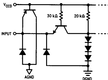
FIGURE 3. Simplified Digital Convert Input Circuit
