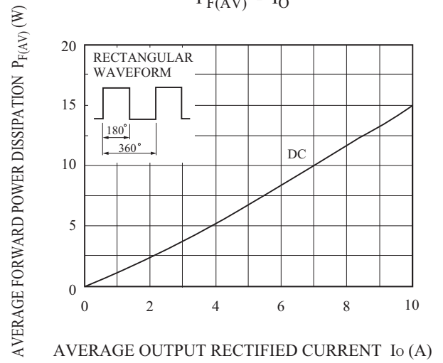
P_{F(AV)} - I_O
