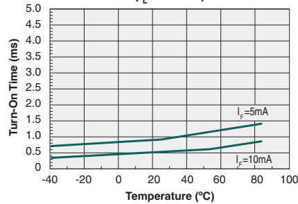
Typical Turn-On Time vs. Temperature ( I_L = 200\text{mA} )
