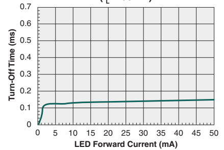
Turn-Off Time vs. LED Forward Current ( I_L = 100\text{mA} )
