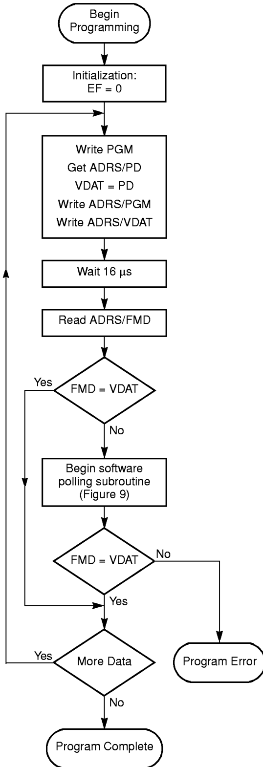
Figure 8. Byte-Wide Programming Flow Chart
