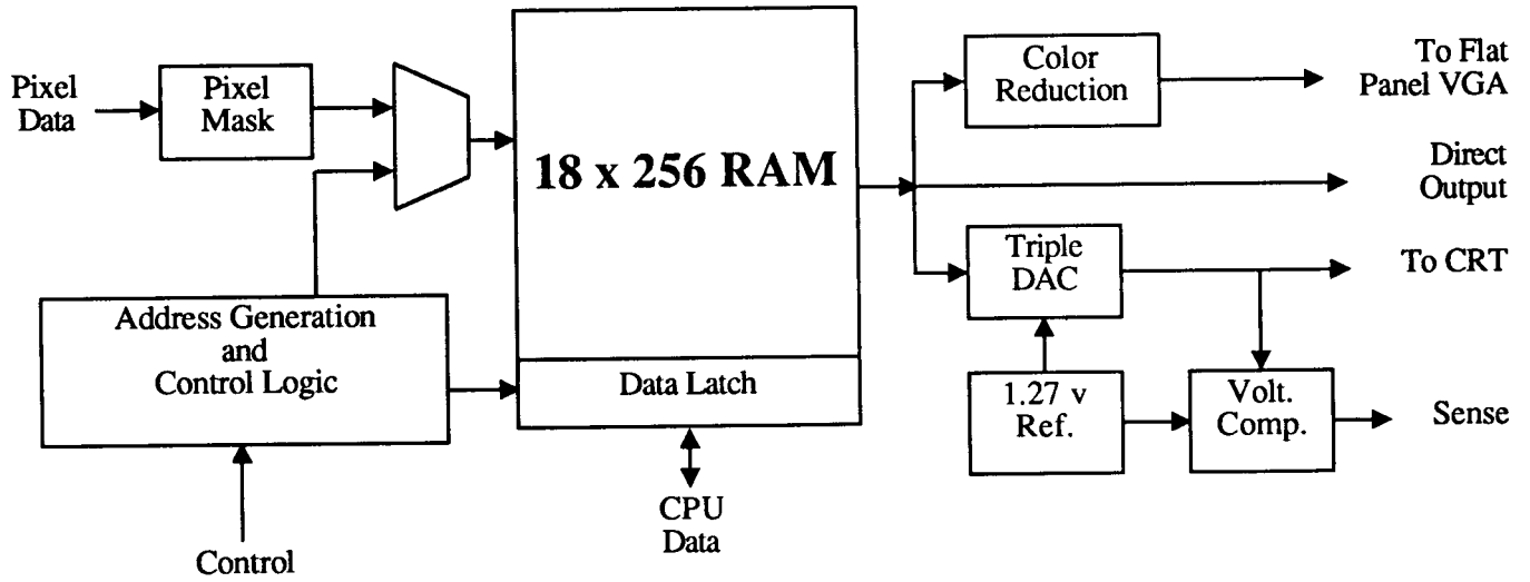
Figure 2-9. 82C411 Block Diagram
