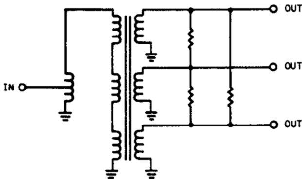
Functional Schematic
