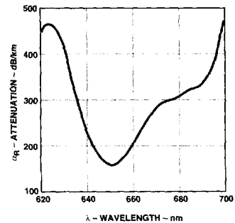
Figure 1. Typical POF Attenuation vs. Wavelength.
