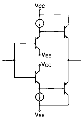
Figure 6: Output Stage
