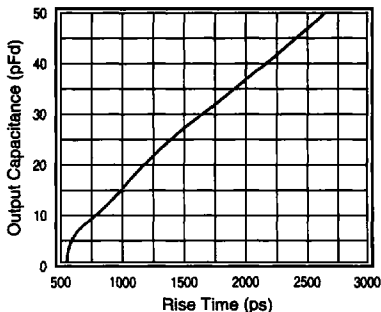
Figure 8. Rise Time vs. C_L
