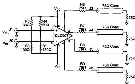
Figure 7: Differential Input DC Coupled Output
