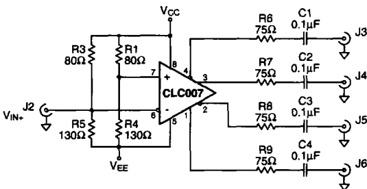
Figure 4: Single Ended 50Ω ECL Input
