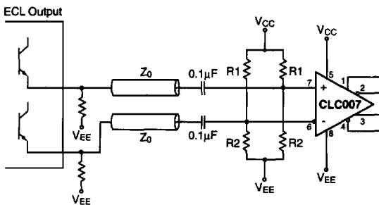
Figure 2: AC Coupled Input
