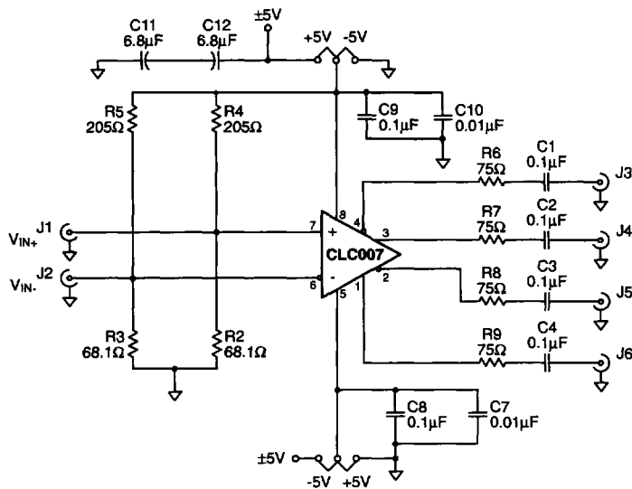
CLC007 Evaluation Board Schematic
