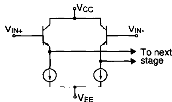
Figure 1: Input Stage
