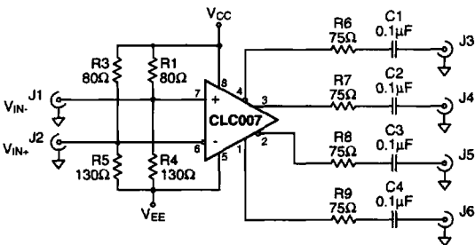
Figure 5: Differential 50Ω ECL Input
