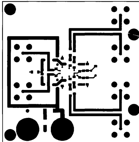
COMLINEAR LAYER2
