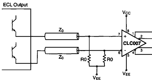
Figure 3: DC Coupled Input
