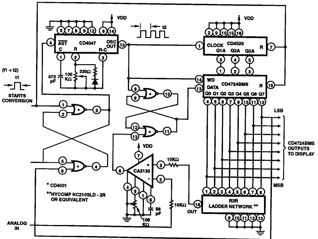
FIGURE 9. A/D CONVERTER
