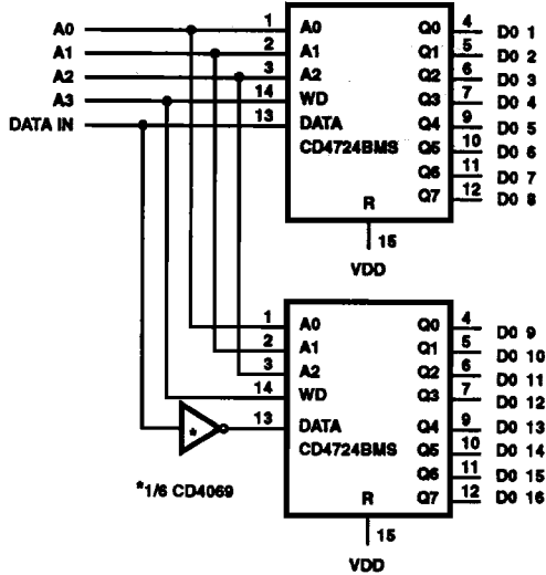
FIGURE 11. 1 OF 16 DECODER/DEMULTIPLER
