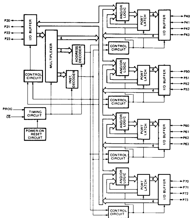
Fig. 2 – BLOCK DIAGRAM
