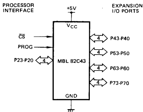
Fig. 1 – LOGIC SYMBOL
