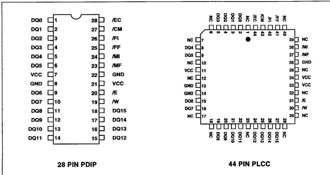
Fig. 2-1 - Pinout Diagrams
