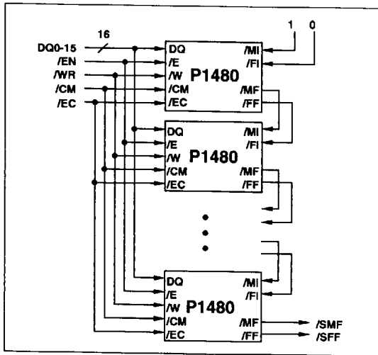
Fig. 3-4 - Vertically Cascaded LANCAMS
