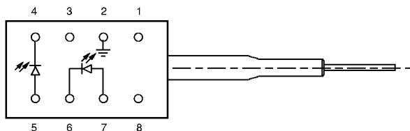
Figure 1. D571-Type Digital Uncooled DFB FastLight Laser Module Schematic, Top View
