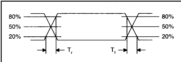
Figure 11. Serial Input Rise and Fall Time
