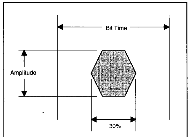
Figure 15. Receiver Input Eye Diagram Jitter Mask
