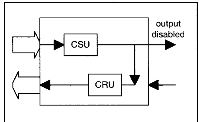
Figure 3. Loopback Operation
