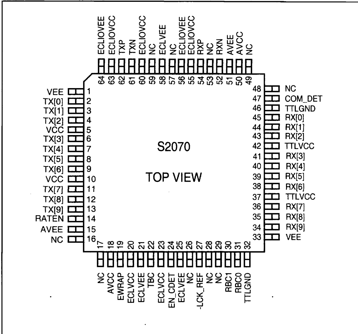
Figure 4. S2070 Pinout
