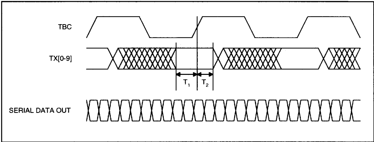
Figure 8. Transmitter Timing
