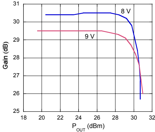
Gain vs. P_{OUT} @ 14 GHz, P_{IN} = -10\text{ dBm} V_{DD} = 8\text{ V} , I_{CQ} = 450\text{ mA} & V_{DD} = 9\text{ V} , I_{CQ} = 400\text{ mA}
