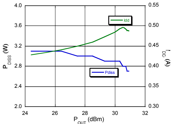
P_{DISS} , I_{DD} vs. P_{out} @ 14.25 GHz
