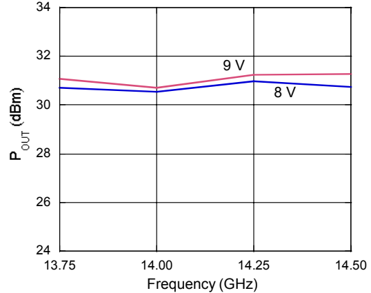
P_{OUT} vs. Frequency @ P_{IN} = -10\text{ dBm} V_{DD} = 8\text{ V} , I_{CQ} = 450\text{ mA} & V_{DD} = 9\text{ V} , I_{CQ} = 400\text{ mA}
