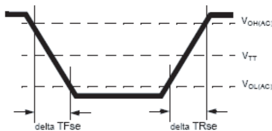
Single-ended Output Slew Rate definition
