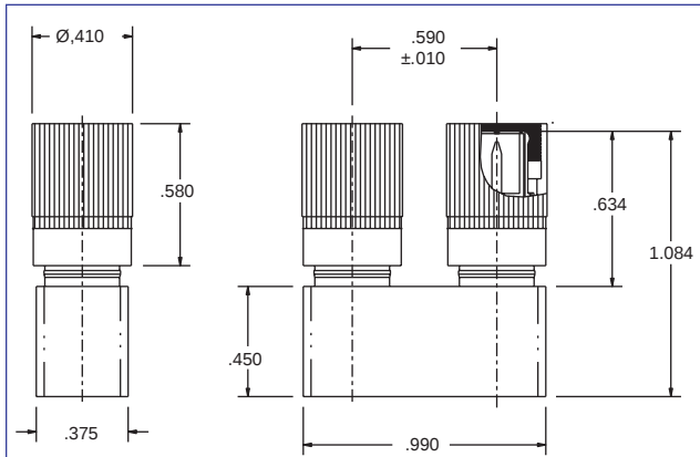
DUAL COAXIAL DIN CONNECTOR "U-LINK" 75 OHM WITH TWO PLUGS BASED ON THE 169-13 SPECIFICATION
