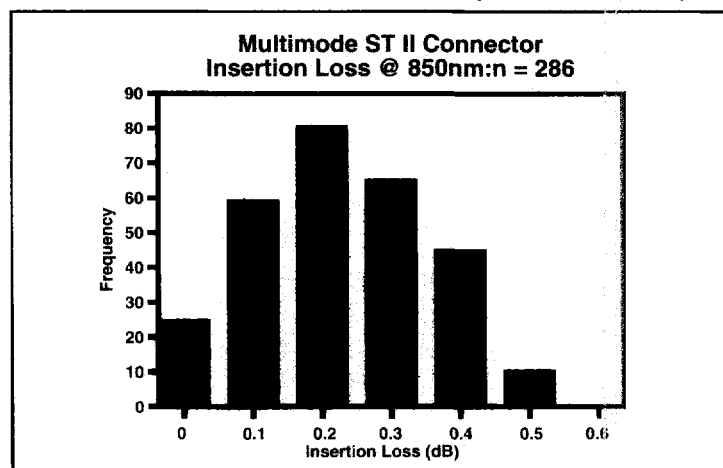
ST Connector 953-101-5310 (62.5/125 fiber)
