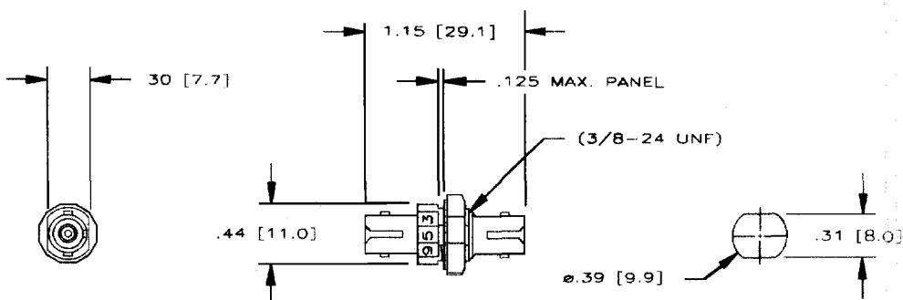
ST II Adapter
