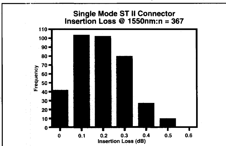
ST Connector 953-101-5306 (9/125 Fiber)
