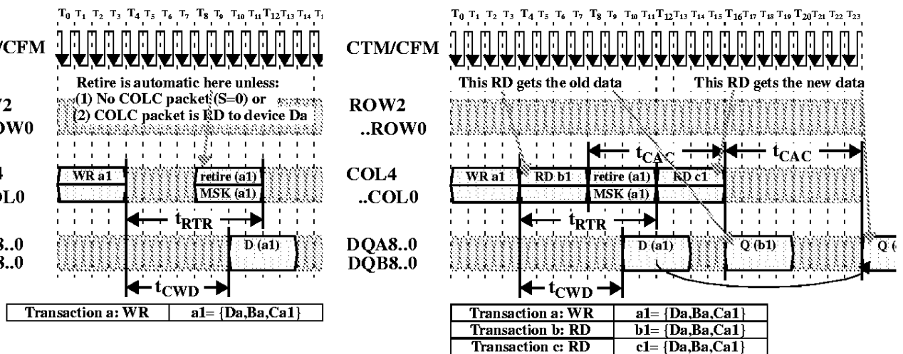
Figure 17: Normal Retire (left) and Retire/Read Ordering (right)
