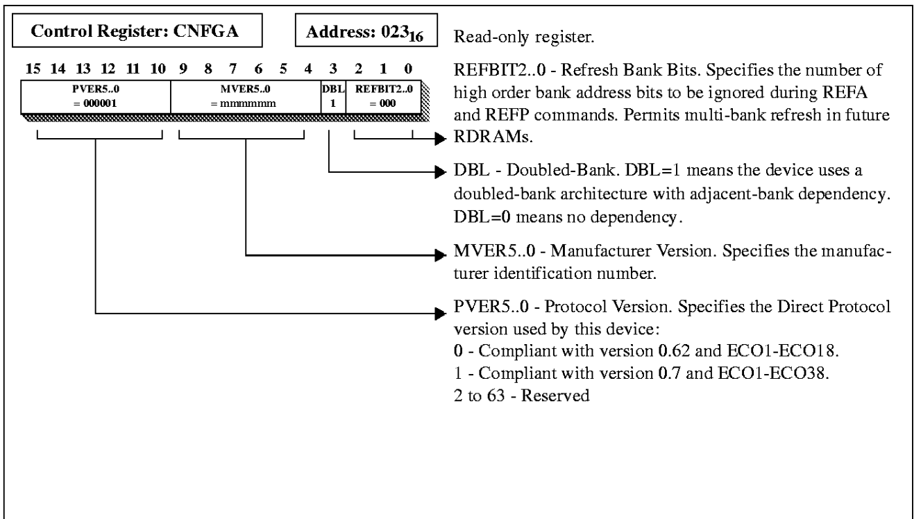
Figure 28: CNFGA Register
