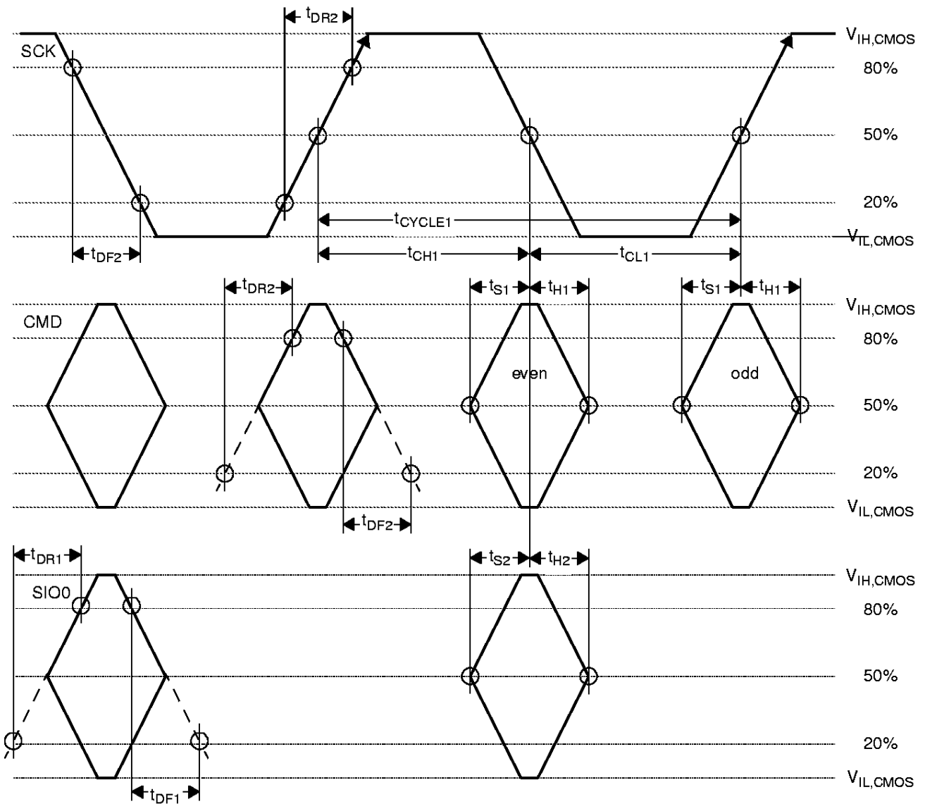
Figure 55: CMOS Timing - Data Signals for Receive
