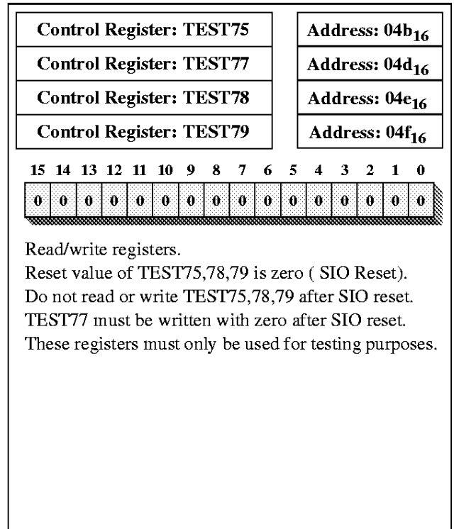
Figure 43: TEST Registers
