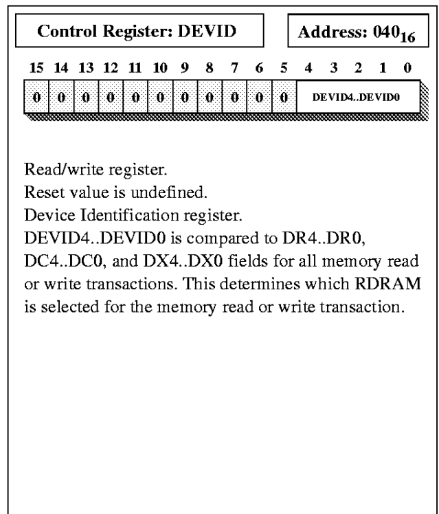
Figure 31: DEVID Register
