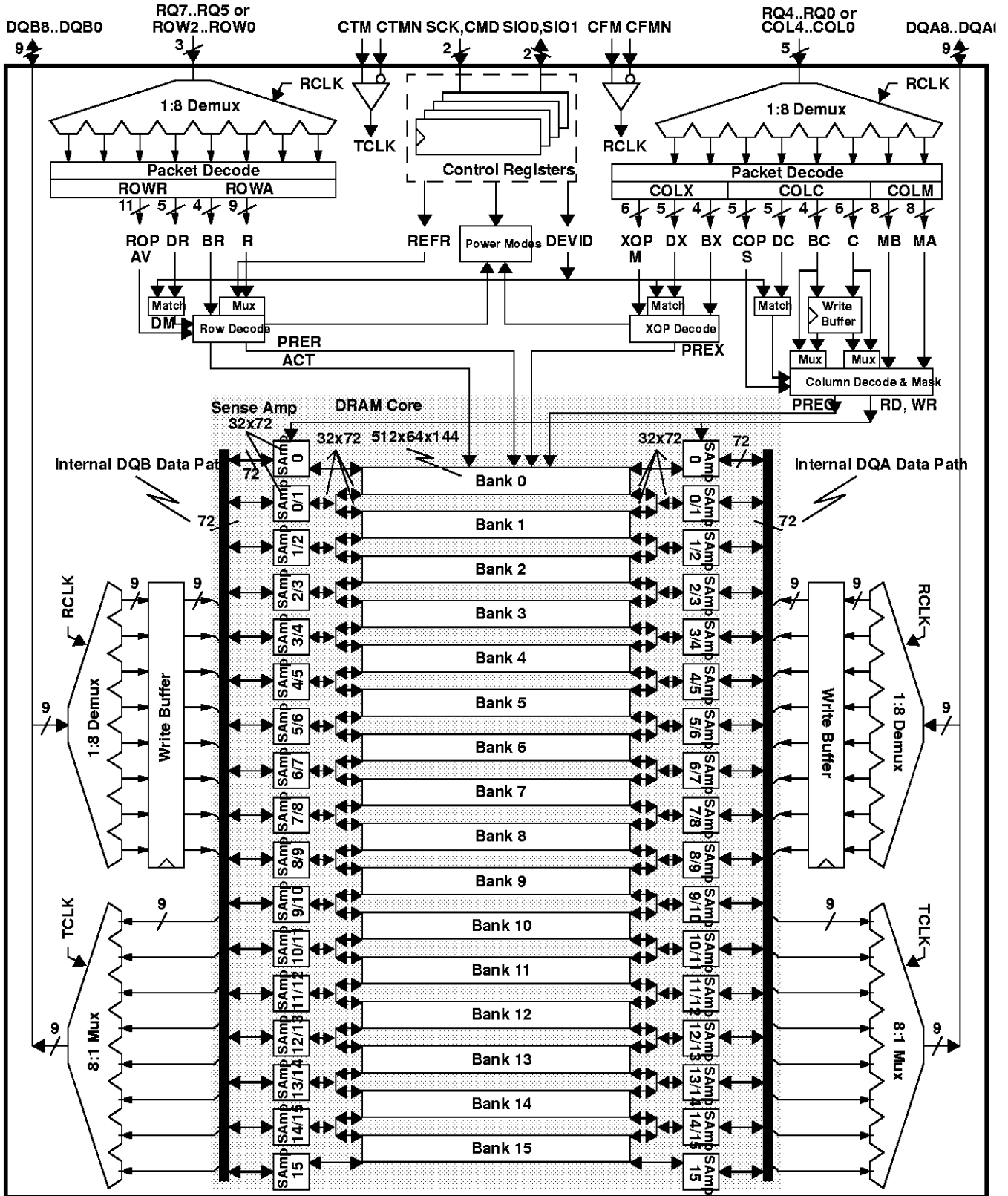
Figure 2: 64/74Mbit Direct RDRAM Block Diagram
