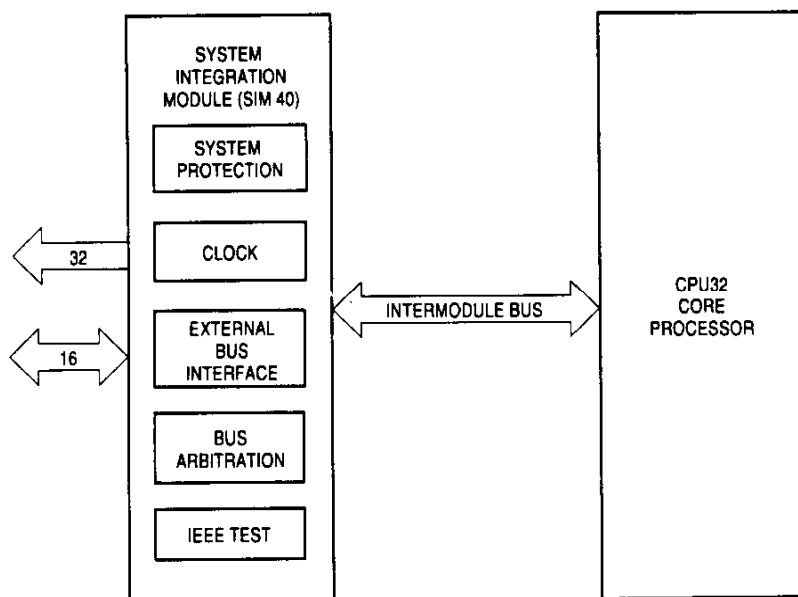
Figure 1. MC68330 Simplified Block Diagram
